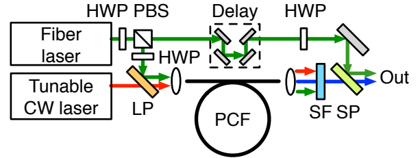
Fig. 3. (Color online) Experimental setup. HWP: half-wave plate, PBS: polarizing beamsplitter, LP: long-pass dichroic mirror, SF: filters (Thorlabs DMSP1000, Chroma HQ735LP), SP: short-pass dichroic mirror.
