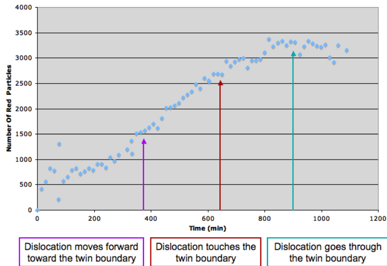
Figure 4.14: Top: the number of particles in the stacking fault bounded by the moving dislocation as a function of time. Bottom: the crystal growth with the dislocations major movements indicated.
