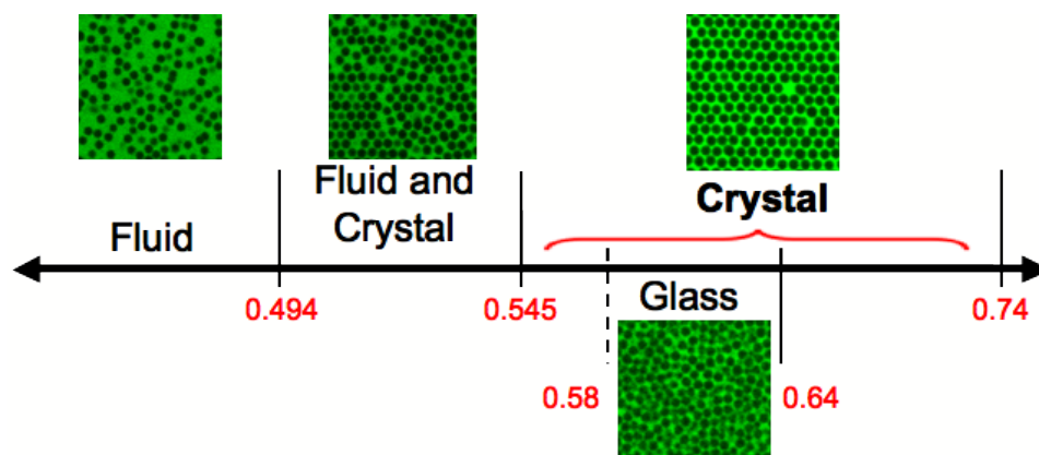
Figure 2.1: A phase diagram for hard sphere colloidal crystals. As the volume fraction, \phi , increases the colloid solution goes from a fluid phase to fluid-crystal coexistence at \phi=0.494 and to a crystalline phase at \phi=0.545 . If the colloids are compressed together quickly (by centrifugation) with the right boundary conditions in a template, an amorphous structure can be obtained above \phi=0.58 . The most close-packed amorphous structure has a \phi=0.64 .
