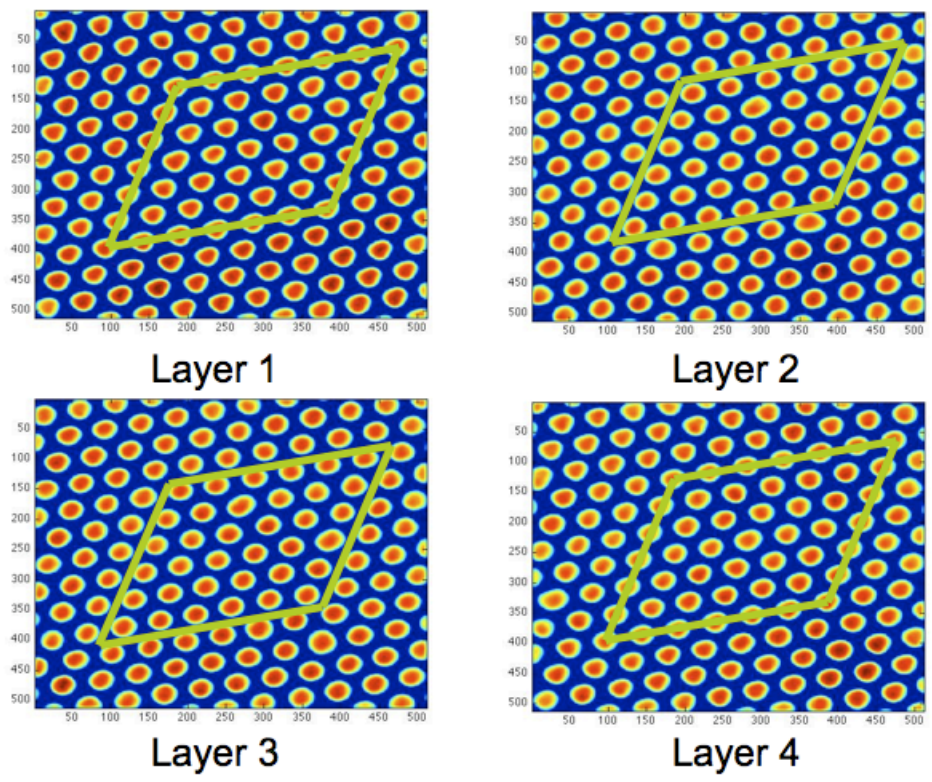
Figure 3.7: A box with known volume drawn onto the four layers in the "zoomed-in" \{111\} crystal. The number of particles in the box is 108.
