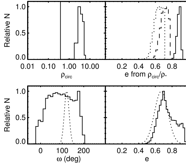
Figure 5.5.—: Posterior distributions of e and \omega for the HD 17156 transiting system, with eccentricity fixed at 0 (row 1) and free to vary (row 2). Row 1: Left: \rho_\star derived from circular fit. The solid line marks the nominal value. Right: Posterior distribution for eccentricity solving Equation (5.5) for \omega = 0 (solid line), \omega = 45^\circ (dashed line), and \omega = 90^\circ (dotted line). Row 2: Left: Posterior distribution for \omega from eccentric fit (i.e. a fit to the light curve in which the eccentricity is a free parameter; solid). Gaussian illustrating posterior from Fischer et al. (2007) RV fit (dotted line). Right: Same for eccentricity posterior.
