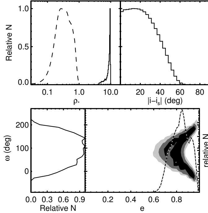
Figure 6.8.—: Top left: \rho_{\text{circ}} obtained from circular fit to the transit light curve (solid) and posterior for \rho_{\star} from Section 6.3.3 (dashed); since the host star is not highly dense (i.e. the two posteriors do not overlap), the planet’s orbit must be highly eccentric. Top right: Posterior for projected spin-orbit alignment from an eccentric fit to transit light curve, imposing a prior on \rho_{\star} . Bottom left: Posterior distribution \omega from an eccentric fit to transit light curve, imposing a prior on \rho_{\star} . Bottom right: Joint posterior for \omega vs. e . The black (gray, light gray) contours represent the \{68.3, 95, 99\}\% probability density levels (i.e. 68% of the posterior is contained within the black contour) Over-plotted as a black-and-white dotted line is a histogram of the eccentricity posterior probability distribution marginalized over \omega .
