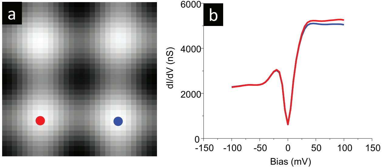
Figure 3.4.2: (a) 2 \times 2 average supercell from T_c=35 K underdoped Bi-2201 with Pb dopants used to suppress the supermodulation. (b) Average spectra from the two inequivalent Bi sites show identical gap energy.
