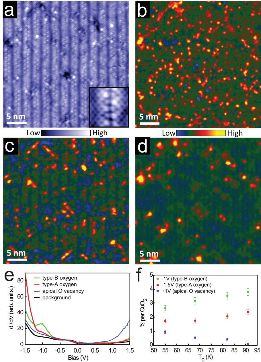
Figure 4.2.1: (a) Atommally resolved topographic image of Bi-2212 with T_c = 55 K, acquired at V_{sample} = +1 V and setpoint current I = 150 pA over a 35 nm area (inset, 3 times magnification). (b-d) dI/dV images in the same area as (a), acquired at V_{sample} = -1, -1.5, and +1 V, respectively. (e) dI/dV spectra over each dopant type, from the T_c=82 K sample. Each colored spectrum is the average of all imaged dopants of its type within a 30-nm field of view; the black trace shows the average spectrum far from dopants. Setup condition: 260 pA and -650 mV. (f) Density of each type of dopant imaged within four samples studied.
