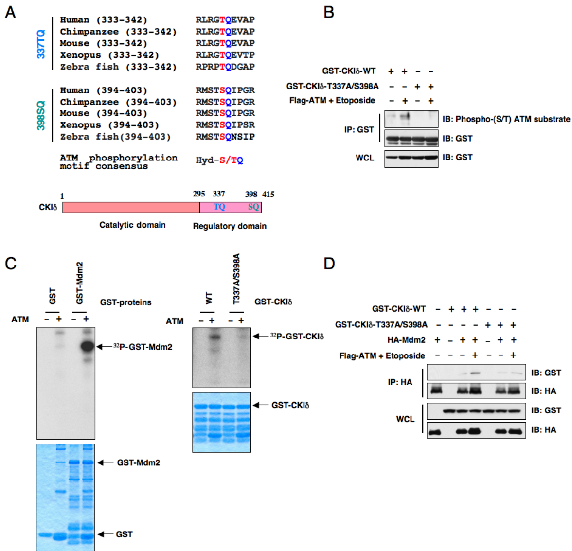
Figure 3: ATM phosphorylates Casein Kinase Iδ to regulate its subcellular localization and its ability to interact with Mdm2. (A) Protein sequence illustration of the two putative ATM phosphorylation sites present in the C-terminus of CKIδ across different species. Hyd: hydrophobic amino acids. (B) Immunoblot analysis (IB) of whole cell lysates (WCL) and immunoprecipitates (IP) derived from 293T cells transfected with the indicated GST-CKIδ constructs in the presence or absence of Flag-ATM. Where indicated, the ATM kinase was activated by treatment with etoposide for 30 minutes before harvesting. The phosphorylation status of CKIδ by ATM in vivo was detected with a specific phospho-(S/T) ATM substrate antibody. (C) ATM phosphorylates both Mdm2 and CKIδ in vitro . The ATM kinase was purified by Flag-immunoprecipitation from 293T cells, and then incubated with 5 μg of GST-Mdm2 or the indicated GST-CKIδ proteins (with GST protein as a negative control) in the presence of γ- 32 P-ATP. The kinase reaction products were resolved by SDS-PAGE and phosphorylation was detected by autoradiography. (D) Immunoblot (IB) analysis of whole cell lysates (WCL) and immunoprecipitates (IP) derived from 293T cells transfected with HA-Mdm2 and the indicated GST-CKIδ constructs. Thirty hours post-transfection, cells were pretreated with 10 μM MG132 for 2 hours to block the proteasome pathway and then treated with 25 μM etoposide (or DMSO as control) for 1.5 hours before harvesting.
