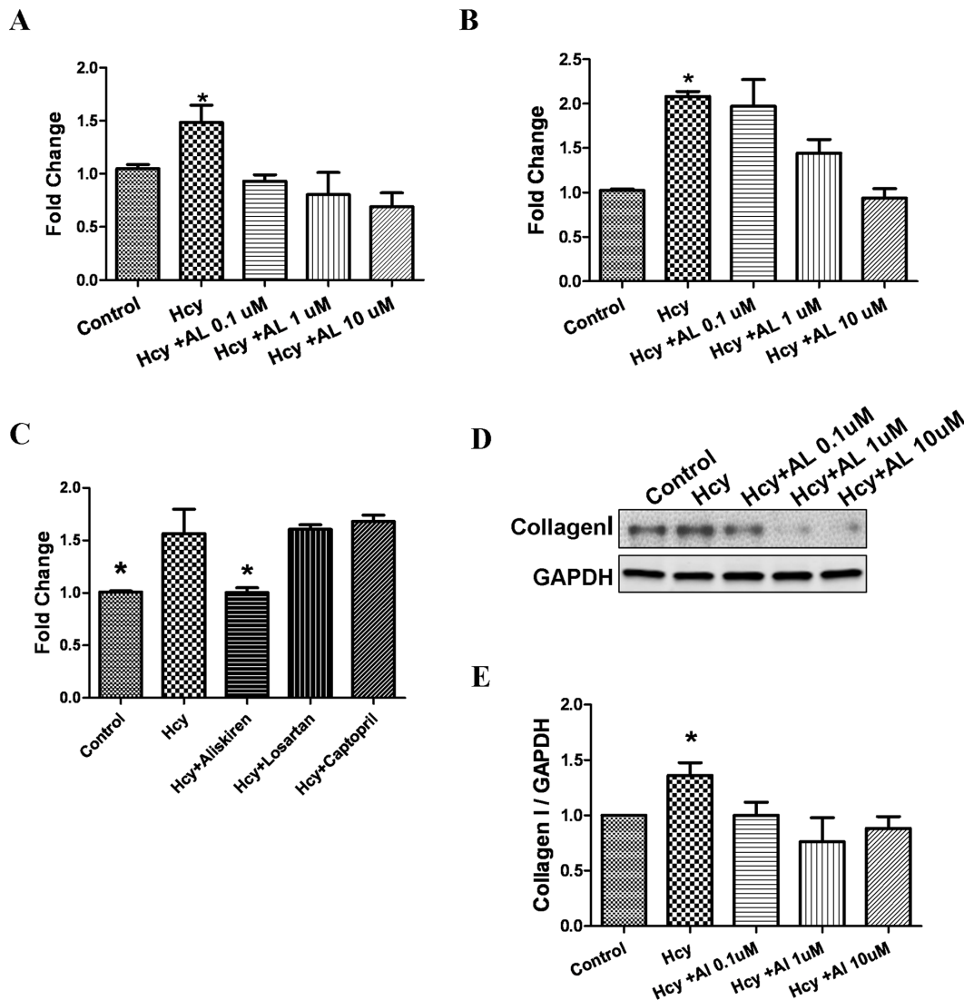
Figure 5. Effects of aliskiren on homocysteine-induced matrix expression in cultured cardiac fibroblasts. Fibroblasts were cultured in the presence or absence of D,L, homocysteine 200 \mu\text{mol/L} for 24 hours after pretreatment with varying concentrations of aliskiren (0.1–10 \mu\text{mol/L} ). Real time PCR was done to measure relative expression of COL1A2 (alpha 2 chain of type I collagen; A) and COL3A1 (alpha 1 chain of type III collagen; B) genes. Figure 5C demonstrates the results of real time PCR to compare the effects of losartan and captopril with aliskiren on homocysteine induced expression of COL1A2 gene. Western blotting was conducted to measure the expression of collagen type I protein (D and E) Glyceraldehyde 3 phosphate dehydrogenase (GAPDH) was used as internal control. Hcy-D,L, homocysteine; AL-aliskiren; Los – losartan; and Cap – captopril. * p < 0.05 . doi:10.1371/journal.pone.0081612.g005
