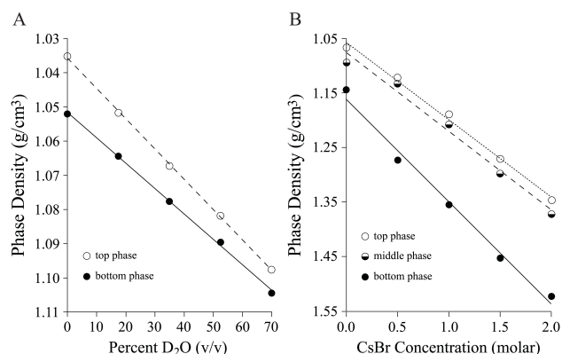
Figure 3. Tuning the density of the phases of MuPS with additives. A two-phase MuPS was prepared from mixtures of PEG and PEOZ in aqueous solutions with a range of isotopic purity (0% to 70% \text{D}_2\text{O} , by volume) (A). A three-phase MuPS was prepared from mixtures of PEG, PEI, and PMAA in aqueous solutions that included CsBr over a range of concentrations of salt (B). In both cases, the densities of the phases increased linearly with the concentration of the additive.
