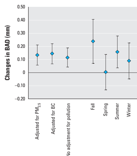
Figure 2. Estimated changes in BAD (in mm) associated with an IQR increase in average daily temperature during the 24 hr before the study visit with and without adjustment for \text{PM}_{2.5} , or BC by season, for baseline BAD (measured before occlusion). Error bars represent 95% CIs.
