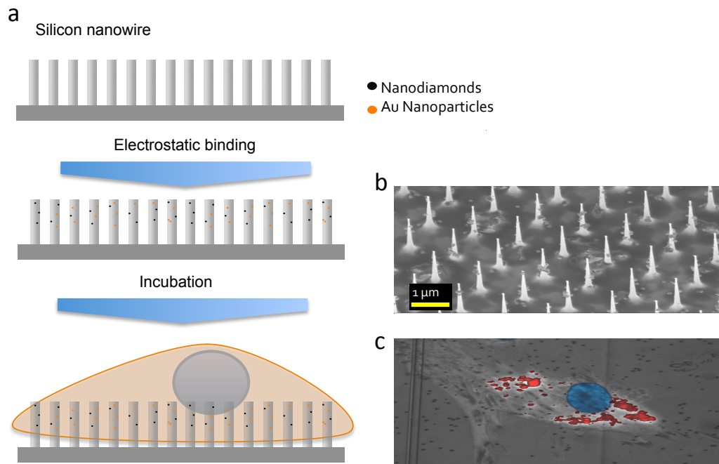
Figure 3.7: | Nano-injection assisted injection of nano-particles into living cells. a , Schematic description of nanoinjection. The array depicts etched silicon nanowires. The small points represent gold colloids and nanodiamonds coated on the nanowire. In the bottom sub-figure a cell with nucleus is grown on the nanowire array. b , Electron microscopy image of a nanowire array coated with gold nanoparticles and nanodiamonds. c , Confocal image of WS1 cell with stained nucleus (blue) and nanodiamonds (red). (credit for image b and c : Minako Kubo)
