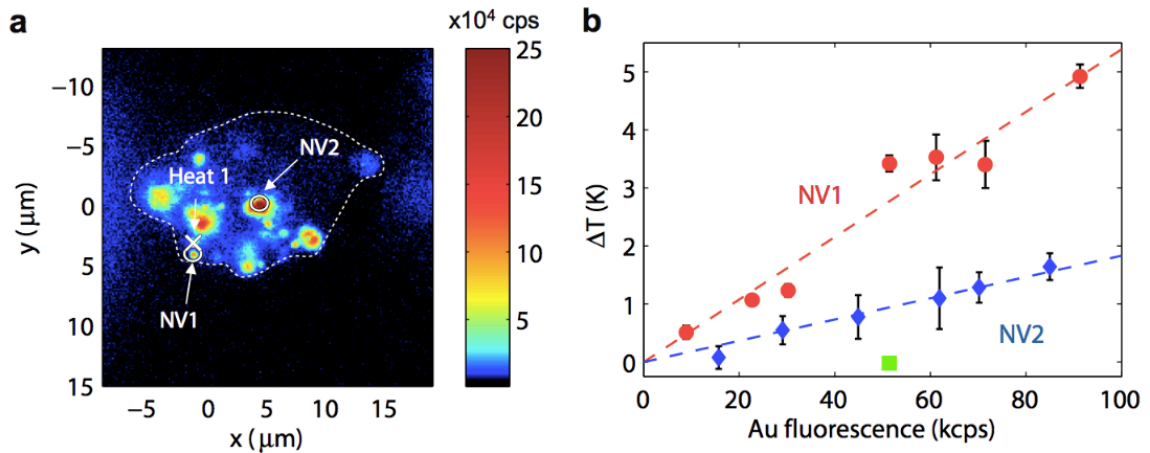
Figure 3.8: | Nanoscale thermometry in cells. a , Confocal scan of a single cell under 532 nm excitation with collection above 638 nm. The cross corresponds to the position of the gold nanoparticle used for heating, while circles represent the location of the nanodiamonds ( NV_1 and NV_2 ) used for thermometry. The dotted line provides a guide to the eye and outlines the cell membrane. Color bars indicate the fluorescence in cps. b , Measured change in temperature at the position of NV_1 and NV_2 relative to the incident laser power applied to the gold nanoparticle. Dashed lines are linear fits to the data. Each point consists of an average of 5 measurements with each individual measurement taking 4 seconds. The error bars (one standard deviation) are set by fluctuations in the laser heating of the gold nanoparticle.
