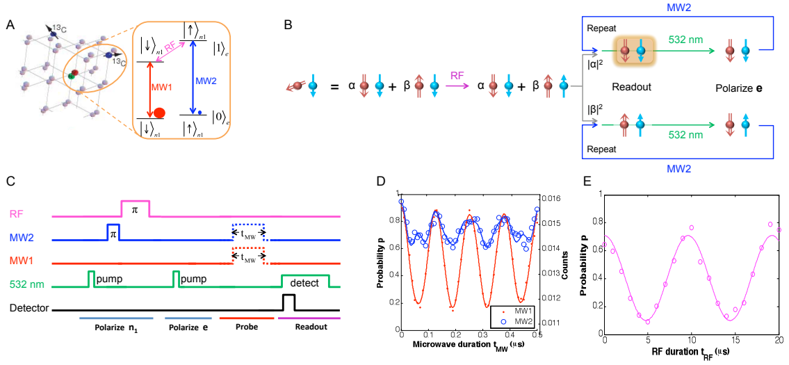
Figure A.1: | Repetitive readout of an electronic spin. (A) Illustration of the NV center and its proximal ^{13}\text{C} nuclear spins. Inset: Energy levels of the coupled spin system formed by the NV electronic spin ( \mathbf{e} ) and the first proximal ^{13}\text{C} nuclear spin ( \mathbf{n}_1 ). With a static magnetic field applied along the NV axis, spin \mathbf{n}_1 keeps the same quantization axis when spin \mathbf{e} is |0\rangle_e or |1\rangle_e . When spin \mathbf{n}_1 is |\downarrow\rangle_{n_1} (or |\uparrow\rangle_{n_1} ), the microwave field MW1 (or MW2) resonantly drives spin \mathbf{e} between |0\rangle_e and |1\rangle_e , which can implement the C_{n_1}\text{NOT}_e gate. When spin \mathbf{e} is |1\rangle_e , the radio-frequency RF field resonantly drives spin \mathbf{n}_1 between |\downarrow\rangle_{n_1} and |\uparrow\rangle_{n_1} , which can implement the C_e\text{NOT}_{n_1} gate. (B) Illustration of repetitive readout. The red down (up) arrow represents the electronic spin state |0\rangle_e ( |1\rangle_e ), and blue down (up) arrow represents the nuclear spin state |\downarrow\rangle_{n_1} ( |\uparrow\rangle_{n_1} ). (C) Experimental pulse sequences that polarize spin \mathbf{n}_1 to |\downarrow\rangle_{n_1} and spin \mathbf{e} to |0\rangle_e , followed by various probe operations, before fluorescence readout of spin \mathbf{e} . (D) Measured electronic spin Rabi oscillations driven by MW1 and MW2 fields, for polarized spin \mathbf{n}_1 . The small wiggles for MW2 are due to off-resonant driving of the majority population in the |\downarrow\rangle_{n_1} state. The data is in agreement for finite detunings and microwave power (solid curves). The right vertical axis shows the average counts for a single readout. The left vertical axis shows the probability in the |0\rangle_e state, obtained from the average counts. (E) Measured nuclear spin Rabi oscillation driven by the RF field.
