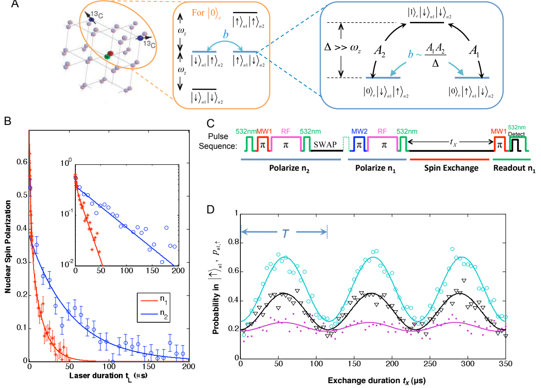
Figure A.3: | Coherence and control of two nuclear spins. (A) The coupled spin system formed by the NV electronic spin ( \mathbf{e} ) and two proximal ^{13}\text{C} nuclear spins ( \mathbf{n}_1 and \mathbf{n}_2 ). Middle inset: Energy levels for spins \mathbf{n}_1 and \mathbf{n}_2 when spin \mathbf{e} is in the |0\rangle_e state. Right inset: Schematic of flip-flop between spins \mathbf{n}_1 and \mathbf{n}_2 , which is electron-mediated by the second-order hopping via |1\rangle_e |\downarrow\rangle_{n_1} |\downarrow\rangle_{n_2} . (B) Measured depolarization of spins \mathbf{n}_1 and \mathbf{n}_2 under optical illumination. For the duration of optical illumination t_L longer than 1 \mu\text{s} , the polarizations for spins \mathbf{n}_1 and \mathbf{n}_2 decay exponentially with characteristic times \tau_{n_1} = 13 ( 1 ) \mu\text{s} and \tau_{n_2} = 53 ( 5 ) \mu\text{s} , respectively. For t_L less than 1 \mu\text{s} , the decay is slightly faster, which is likely associated with dynamics of the spin-fluctuator model that describe optically induced depolarization of single nuclei [67]. These decay times are much longer than the optical readout/pump time of the electronic spin (about 350 ns). Inset: Log-linear plot. (C) Operations and pulse sequence to probe dynamics between spins \mathbf{n}_1 and \mathbf{n}_2 . (D) Measured spin flip-flop dynamics between spins \mathbf{n}_1 and \mathbf{n}_2 . For three different preparations of the initial state ( |\downarrow\rangle_{n_1} |\uparrow\rangle_{n_2} (cyan), |\downarrow\rangle_{n_1} and n_2 in thermal state (black), and |\downarrow\rangle_{n_1} |\downarrow\rangle_{n_2} (purple)), the observed population, p_{n_1, \uparrow}(t) , oscillates with the same period T = 117 ( 1 ) \mu\text{s} . These observations verify the theoretical prediction, with flip-flop coupling strength b = 4.27 ( 3 ) kHz.
