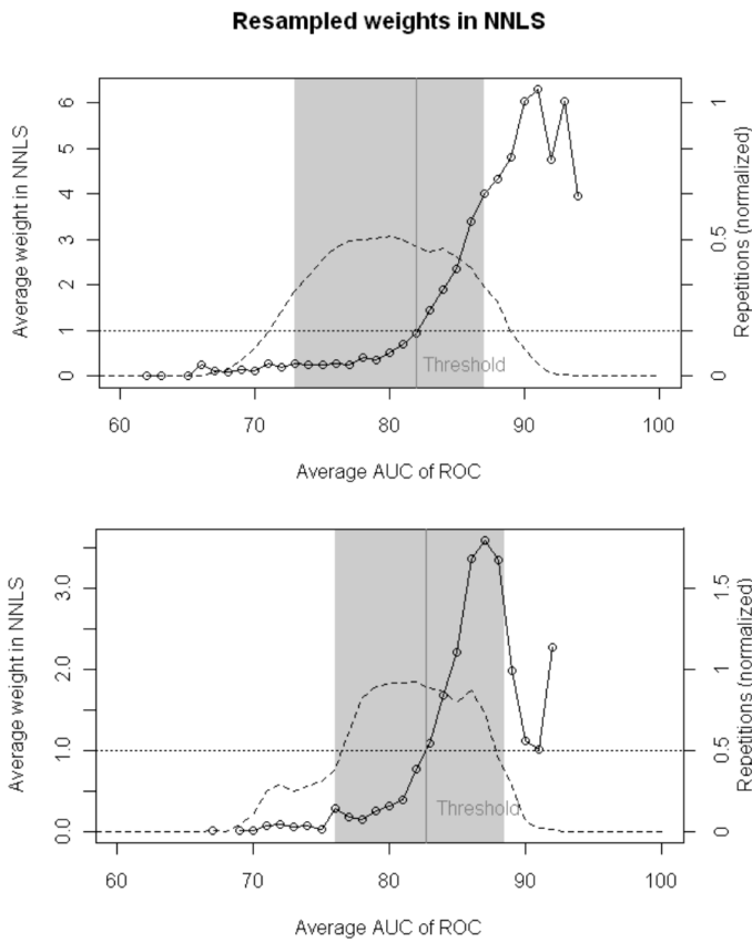
Fig. 10. Learning the relation between weight and data quality for the western (top) and eastern (bottom) test area. Shown is the weight function used when averaging the probability maps, the distribution of the available observations with inner 75% quantile (dark gray).
