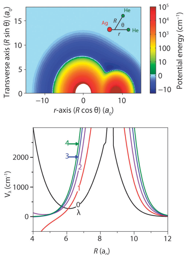
Fig. 11 Top: Pairwise \text{AgHe}_2 interaction PES, evaluated at r = 8.75 a_0 , corresponding to the bottom of the AgHe potential well. Color scale is logarithmic, with green to red indicating energies from 1 to 10^5 \text{ cm}^{-1} , and cyan to blue indicating energies from -1 to -15 \text{ cm}^{-1} . Bottom: Lowest-order expansion coefficients V_\lambda(R) of the \text{AgHe}_2 PES as functions of R , evaluated with r = 8.6 a_0 . Note the divergence in the vicinity of R = 8.5 a_0 .
