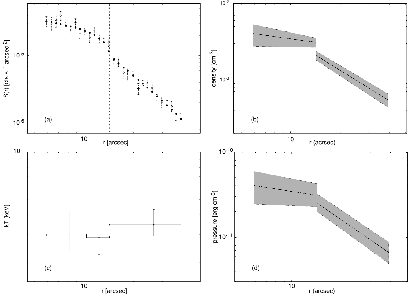
Figure 5. Shock in 3C 288 showing the eastern edge (sector between P.A. = 30° and P.A. = 130°). Panel (a) shows X-ray surface brightness profile. The filled circles are the model values that correspond to the best-fit gas density model shown in panel (b). Panel (c) shows the temperature profile. Panel (d) shows the pressure profile obtained from the temperatures on either side of the edge and density profile. Error bars are 90%; the vertical dashed line in panel (a) shows the position of the density jump.
