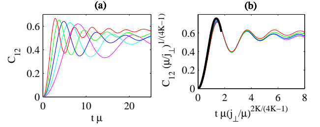
FIG. 4: [Color online] Truncated Wigner approach (11). (a) Numerical results for j_{\perp}/\mu = 0.27 (red), 0.16 (green), 0.10 (blue), 0.060 (cyan), 0.036 (magenta) with K = 5 , system size L = 400 , number of random paths M = 400 . (b) Data-collapse according to Eq. (10), superimposed to the result from the series expansion (black curve, identical to Fig. 3(b)).
