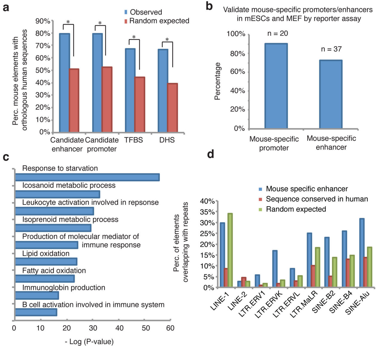
Figure 3. Comparative analysis of the cis elements predicted in the human and mouse genome a. Charts show the fractions of the predicted mouse cis regulatory elements with homologous sequences in the human genome (Methods). b. A bar chart shows the fraction of the DNA fragments tested positive in the reporter assays performed either using the mESC or Mouse embryonic fibroblasts (MEF). c. A chart shows the Gene ontology (GO) categories enriched near the predicted mouse-specific enhancers. d. A bar chart shows the percentage of the predicted mouse-specific enhancers containing various subclasses of LTR and SINE elements. As control, the predicted mouse cis elements with homologous sequences in the human genome or random genomic regions are included.
