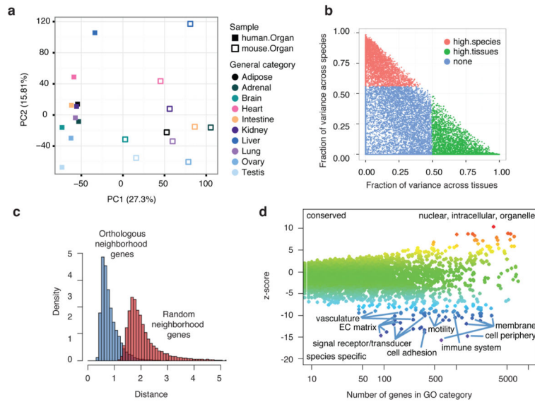
Figure 2. Comparative analysis of the gene expression programs in human and mouse samples a. Principal Component Analysis (PCA) was performed for RNA-seq data for 10 human and mouse matching tissues. The expression values are normalized across the entire dataset. Solid squares denote human tissues. Open squares denote mouse tissues. Each category of tissue is represented by a different color. b. Gene expression variance decomposition (see Method) estimates the relative contribution of tissue and species to the observed variance in gene expression for each orthologous human-mouse gene pair. Green dots indicate genes with higher between-tissue contribution and red dots genes with higher between-species contributions. c. Neighborhood analysis of conserved co-expression (NACC) in human and mouse samples. The distribution of NACC scores for each gene is shown. d. A scatter plot shows the average of NACC score over the set of genes in each functional GO category. Highlighted are those biological processes that tend to be more conserved between human and mouse and those processes that have been less conserved (See Supplementary Table 21 for list of genes).
