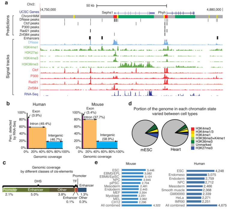
Figure 1. Overview of the mouse ENCODE data sets
