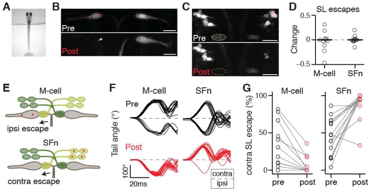
Figure 2.12. Spiral fiber neurons are necessary for lateralized Mauthner-cell-mediated escapes.
