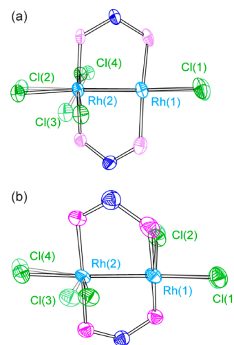
Figure 3. Thermal ellipsoid plots of photocrystallography results with photoinduced structures (solid) superimposed on dark structures (faded). (a) \text{Rh}_2[\text{I,III}] plot; \text{Rh}^1\text{–Rh}^2\text{–Cl}^3 91.05(5)^\circ (dark), 83.2(2)^\circ (photoinduced). (b) \text{Rh}_2[\text{II,II}] plot; \text{Rh}^1\text{–Rh}^2\text{–Cl}^3 91.15(5)^\circ (dark), 78(2)^\circ (photoinduced).
