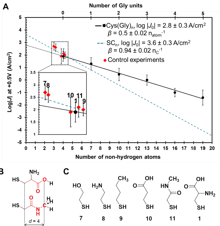
Fig.2. A) Plot of the Gaussian mean values of \log|J| at +0.5 V versus molecular length for oligoglycines (solid line) and n -alkanethiolate standards (dashed line) using a junction with the structure \text{Au}^{\text{TS}}/\text{SAM}/\text{Ga}_2\text{O}_3/\text{EGaIn} . Error bars represent the standard deviation of Gaussian mean values. Molecules that are shorter than cysteine (1), but still possess some structural similarities to it (7, 8), give current densities that fit to the line for n -alkanethiolates (dashed line). B) The molecular length is calculated based on the number of non-hydrogen atoms, starting with carbon next to the sulfur atom, and counting to the final non-hydrogen atom (for example, number of atoms for both Cys (1) and 11 is 4). C) Structure of “short” molecules that are similar in composition to cysteine. The current densities of these molecules were measured to develop a feeling for the reliability of extrapolation as a method of estimating J_0 for the series. \text{Cys(Gly)}_n\text{OH} .
