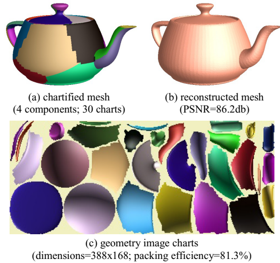
(c) geometry image charts (dimensions=388x168; packing efficiency=81.3%) Figure 11: As opposed to the GIM framework, MCGIMs can represent meshes with multiple components, such as this teapot.
