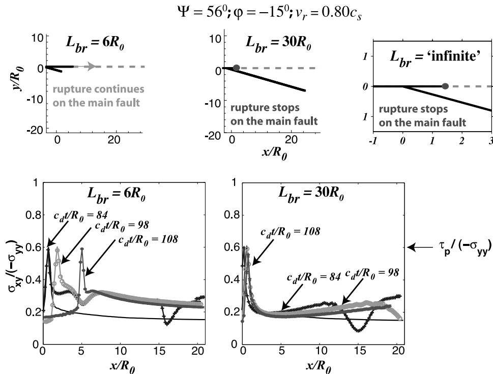
Figure 9. Effect of increasing branch length on the final state of rupture and the corresponding evolution of scaled shear stress distribution on the main fault around the branching junction (stress scaled by fault normal stress, -\sigma_{yy} ) for various time steps (non-dimensionalized as c_d t / R_0 ) for the case when \Psi = 56^\circ , \varphi = -15^\circ and v_r = 0.80c_s . The time steps correspond to time from when the rupture on the main fault is approaching the branching junction to the time when the rupture has completely stopped on the main fault. \tau_p is the peak strength of the fault in the slip-weakening relationship. Here \tau_p / \sigma_{yy} = 0.12 and L_{br} is the length of the branch.
