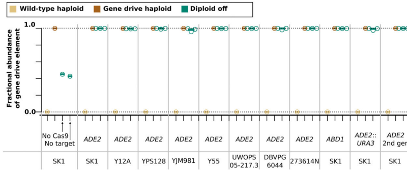
Figure 4. Quantitative PCR demonstrates highly efficient inheritance biasing by split drives across diverse yeast strains in the presence of Cas9. Results depict the relative abundance of wild-type and drive-containing alleles in diploids arising from matings between SK1 haploids bearing gene drives and diverse wild-type haploid strains. “No Cas9” and “No Target” refer to haploid cells containing the ADE2 drive mated to wild-type haploids in the absence of Cas9 or to an otherwise wild-type strain with Cas9 that has a mutation in the targeted sequence that blocks cutting. “2nd gen” refers to the haploid progeny of an earlier mating. Data points are from independent cultures or mating events and represent the mean of 3 technical replicates.
