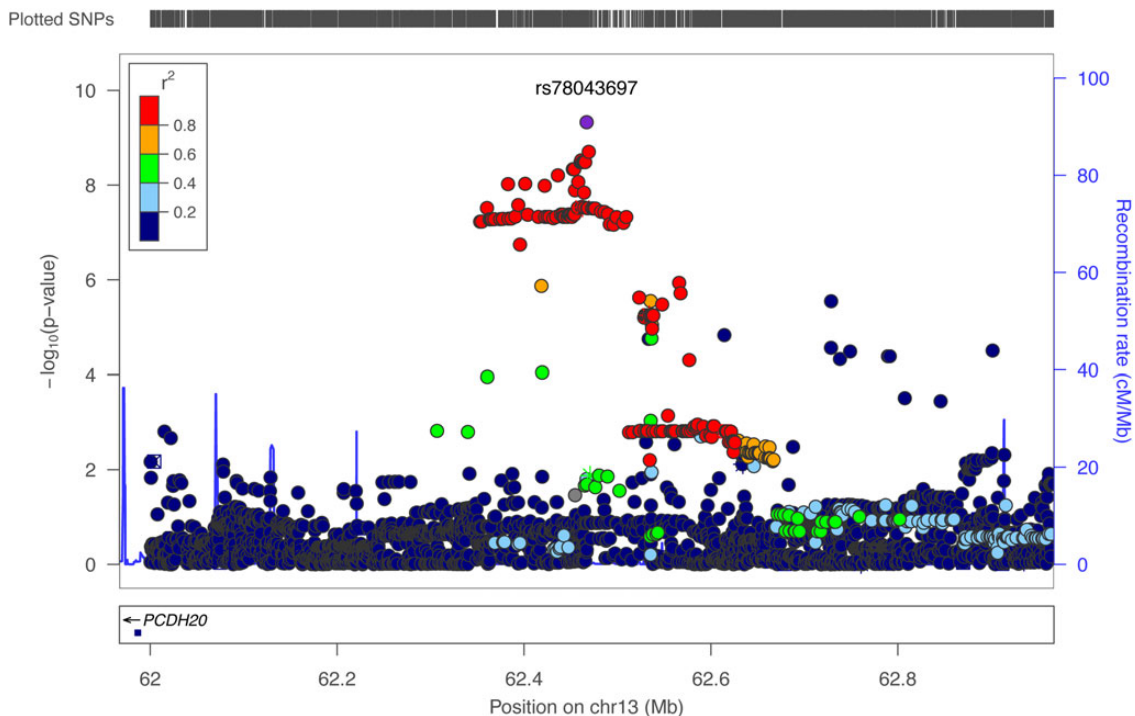
Figure 1. Locus-plot for chromosome 13 locus. The plot shows the locus on chromosome 13 associated with normal hearing functions measured at 2 kHz, highlighting the top SNP rs78043697 and several other significant SNPs in the same region being in high linkage disequilibrium. The results plotted were obtained with a two-stage meta-analysis, focusing on Italian isolates first and then including the communities from the Silk Road. The y-axis shows -\log_{10} of the P-values obtained from the complete meta-analysis of the 2 kHz hearing threshold. The closest gene PCDH20 is shown along the x-axis.
