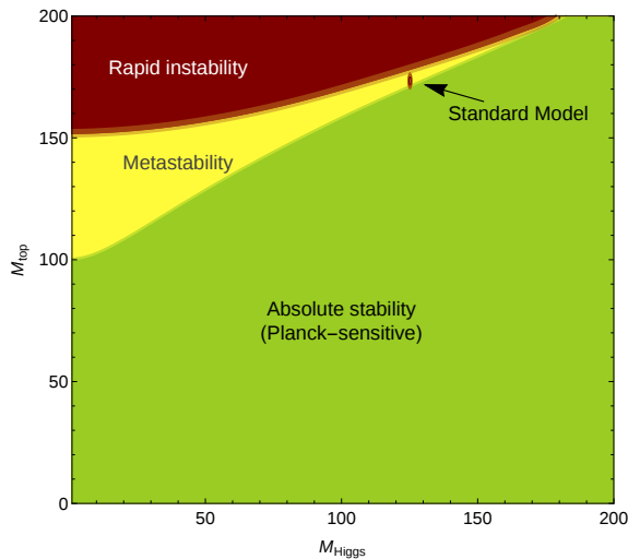
FIG. 5. Same as previous figure but zoomed out. Theory uncertainties on the absolute and metastability bounds are not shown.
