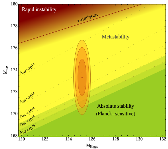
FIG. 4. Boundaries of absolute stability (lower band, NLO) and metastability (upper line, LO). The thickness of the lower boundary indicates perturbative and \alpha_s uncertainty. The theoretical uncertainty of the metastability boundary is unknown. The elliptical contours are 68%, 95% and 99% confidence bands on the Higgs and top masses: m_h^{\text{pole}} = (125.14 \pm 0.23) GeV and m_t^{\text{pole}} = (173.34 \pm 1.12) GeV. Dotted lines are scales in GeV at which V_{\text{min}} can be lifted positive by new physics.
