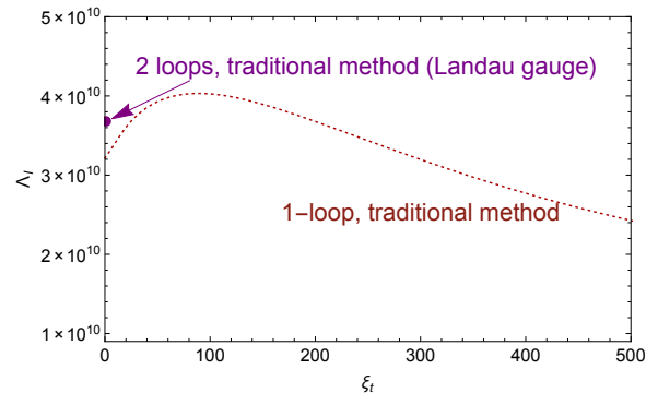
FIG. 2. Gauge dependence of the instability scale \Lambda_I , defined by V(\Lambda_I) = 0 , at 1-loop in the traditional approach. There is no known way to make this scale gauge-invariant.
