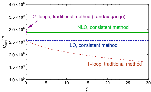
FIG. 3. Gauge dependence of the SM potential at its maximum with m_h^{\text{pole}} = 125.14 GeV and m_t^{\text{pole}} = 173.34 GeV.
