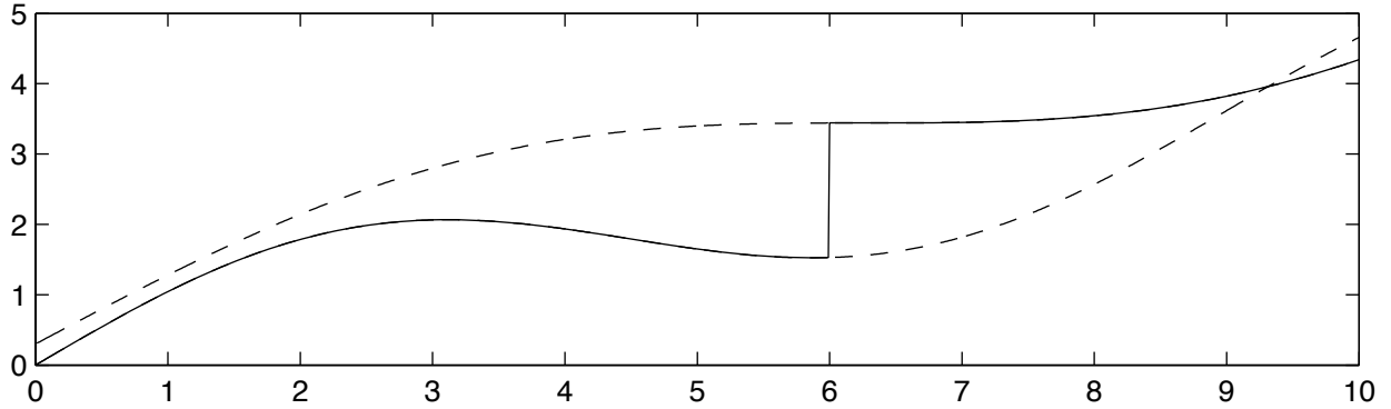
Fig 2: Potential and Observed Outcome Regression Functions
