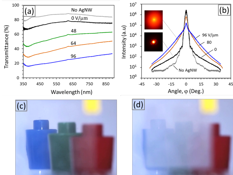
Fig. 3. (a) In-line spectral transmittance for different applied nominal field. There is a slight absorption centered at about 360 nm which is attributed to plasmon resonance in the silver nanowires. (b) Angular distribution of the transmitted laser light (632 nm). The broadening is increased substantially as the surface deforms when the electric field is increased. This is also seen qualitatively in the recorded images in the insert. (c) A demonstration of light scattering is shown by the change in the clarity of the objects placed behind the sheet (c) before and (d) after the application of field of 130 V/μm. Upon removal of field, the sheet immediately returns to its initial, transparent condition. The electrode area is square, as shown by the white opaque area in (d) and is connected to an external power supply through the yellow tab in the upper right. The measurement setups for (a, b) and the real-time video of (c, d) are shown in Fig. S3 and Video 1 in the electronic supplementary information, respectively.
