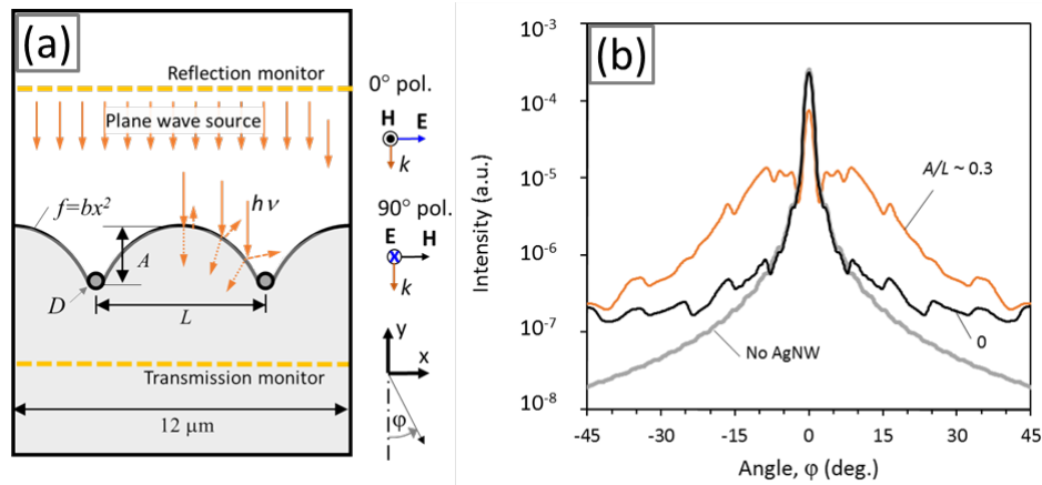
Fig. 4. (a) Schematic of the in FDTD 2D-simulation setup used to calculate angular distribution profile from a regularly spaced, L , parallel nanowires with diameter D , and surface undulations with amplitude A . (b) The results of simulation show the transmission as a function of spread angle, \phi . The transmission is averaged from 4 different spacing ( 1 \mu\text{m} , 2 \mu\text{m} , 6 \mu\text{m} , and 12 \mu\text{m} ) and each at similar relative bulge amplitudes ( A/L \sim 0.3 ).
