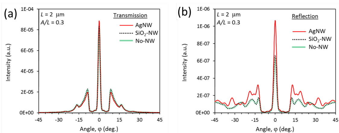
Fig. S2. Comparison of simulated scattering profile in absent of nanowires, just the bulge, (thick green line), with nanowire made of silver (red line), and nanowire made of glass (dotted line) are shown for (a) in transmission and (b) in reflection. At a relatively high bulge amplitude A/L = 0.3 , the scattering from metallic silver structure is negligible in the transmission and more pronounced in the reflection.
