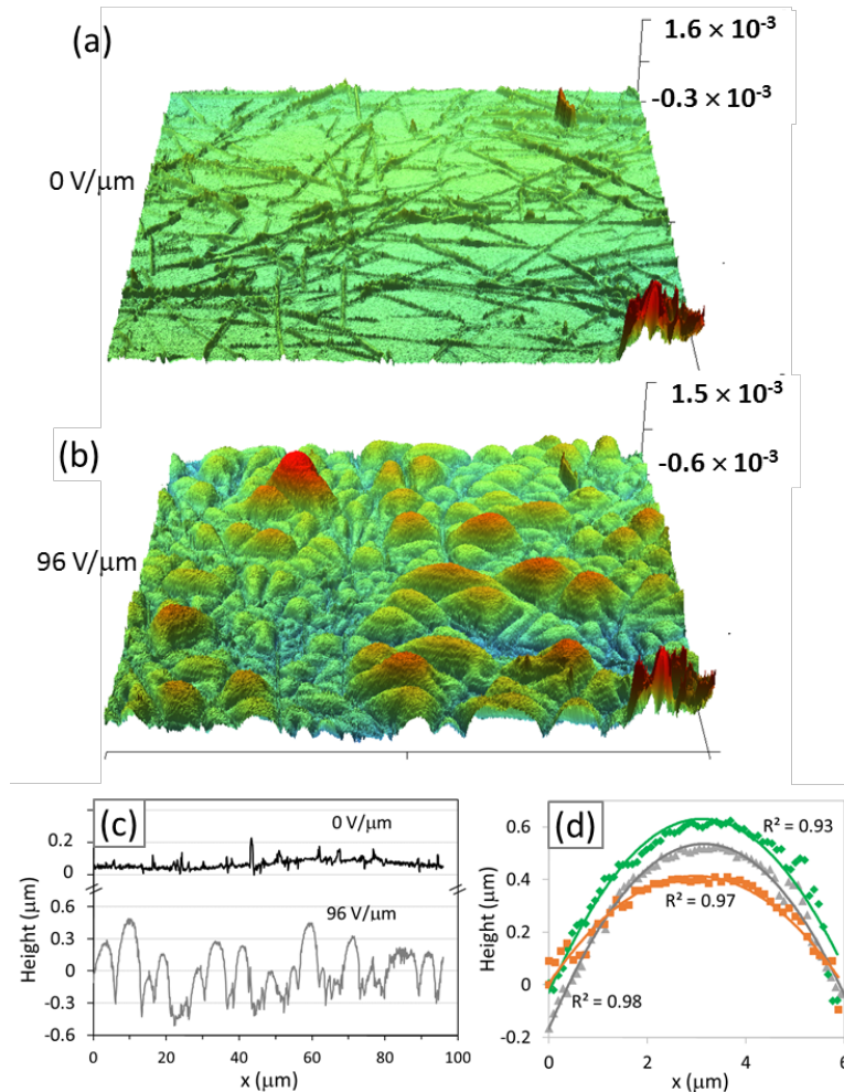
Fig. 2. Confocal microscopy maps of the nanowire electrode and the elastomer surface. (a) without any field and (b) at an applied electric field (nominal) of 96 \text{ V}/\mu\text{m} . The scanned area is 96 \times 96 \mu\text{m}^2 . (c) Line profiles show that the surface morphology is much rougher and in places can be several times the diameter of the silver nanowires (diameter 90\text{nm} ) when the voltage is applied. The dips in the lower trace correspond to the locations of individual nanowires. (d) Detailed fitting of the surface bulges formed between two nearly parallel nanowires. These profiles can be fit reasonably well using parabolic equation (solid lines).
