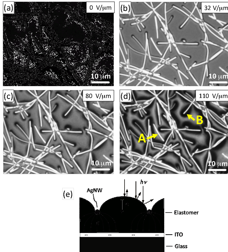
Fig. 1. (a) Bright field optical microscope image showing the spatial distribution of the silver nanowires and the surface of the elastomer in between. The areal density of nanowires is \sim 78 \text{ mg/m}^2 . (b) to (d) the same region at the indicated electric fields (nominal) showing the field-induced local deformations of the elastomer surface revealed by optical contrast change. (e) A schematic cross-section of the surface displacements and the electric field emanating from individual nanowires.
