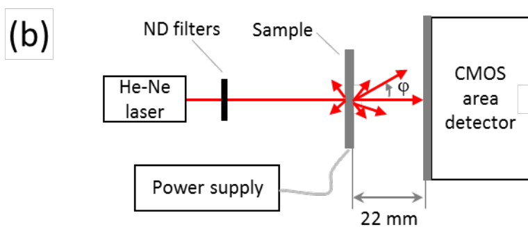
Fig. S1. Schematic of the arrangement for measuring the (a) direct transmittance and (b) angular broadening of the transmitted light.
