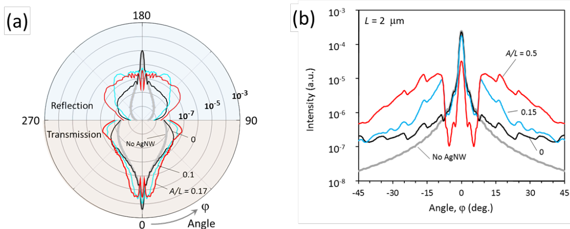
Fig. S3. Example of simulated scattering profile at (a) spacing at L = 6 \mu\text{m} and (b) L = 2 \mu\text{m} . Note that in (a) both transmission and reflection are shown in a polar plot while in (b) only shows the angular dependence in transmission.
