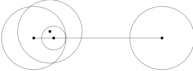
Figure 6. Verifying the strict elder sibling property.
