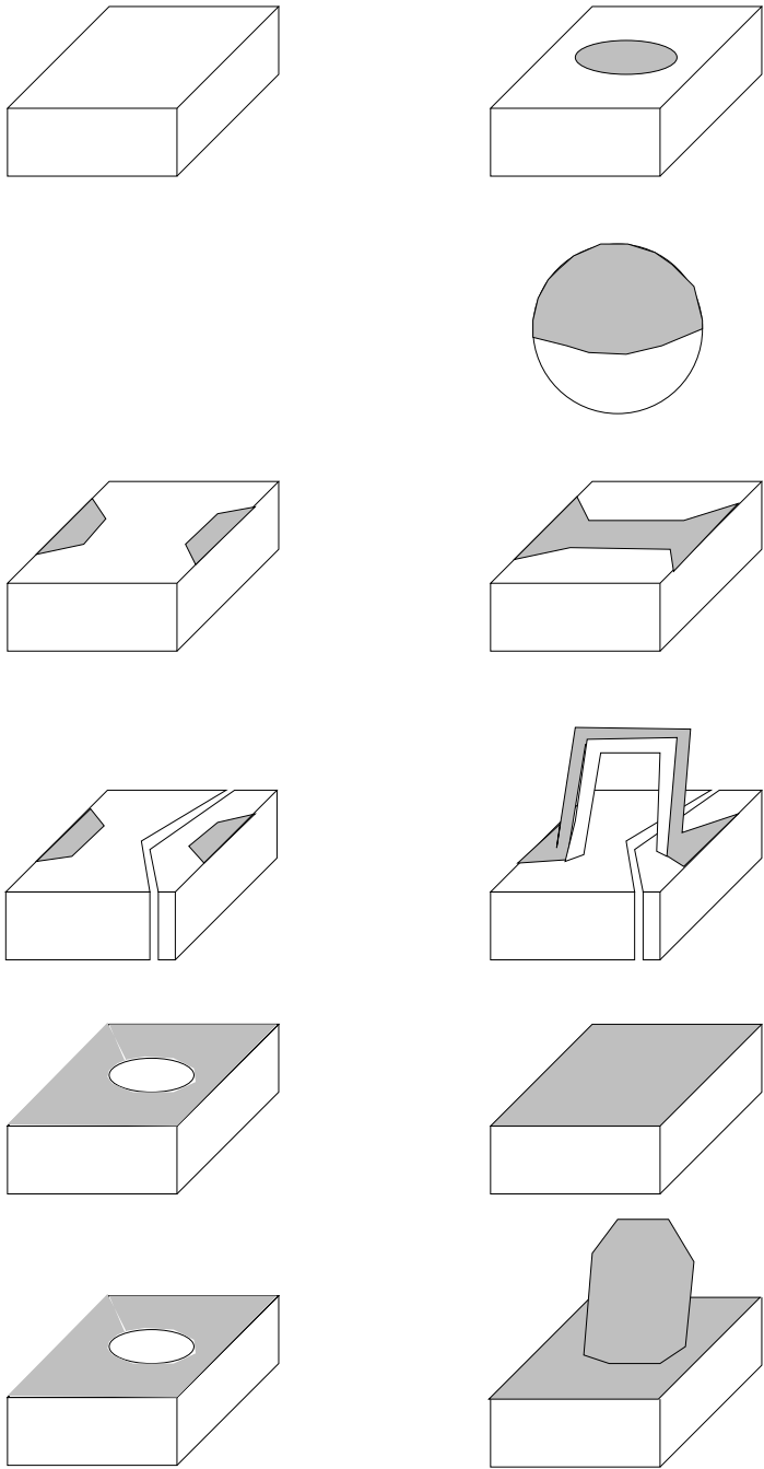
Figure 1. Classification of critical points and handles.
