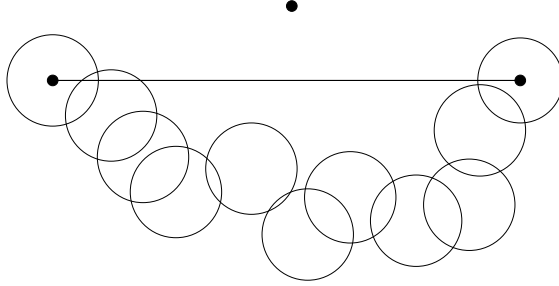
Figure 5. A quasigeodesic chain.
