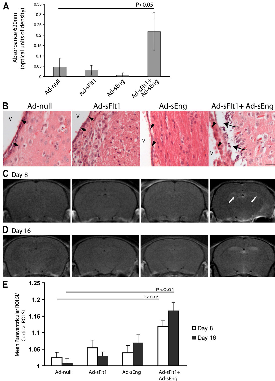
Figure 4. Effect of VEGF and TGF- \beta neutralization on brain permeability. (A) Experimental mice infected for 3 d were injected intravenously with 2% Evans blue in PBS. After 40 min, the brains were removed and quantified for Evans blue/albumin leakage. Simultaneous treatment with sFlt1 + sEng ( n = 3 ) resulted in significantly increased Evans blue leakage into the extravascular space, whereas no changes could be detected with sFlt1 or sEng alone. Values represent means \pm SD. (B) H + E staining of sections of the lateral ventricle of mice expressing sFlt1 + sEng for 14 d revealed marked periventricular edema (arrows) below the ependyma (arrowheads); no edema was observed in this region in other experimental or control mice. V, ventricle. Bar, 25 \mu m. (C and D) T1-weighted coronal MRI of experimental mice intravenously injected with Gd at 8 (C) and 16 (D) d after infection revealed focal lesions surrounding the lateral ventricles in the midcortex of mice expressing sFlt1 + sEng (white arrows) but not in the other experimental groups. (E) Quantification of the ratio of signal intensity in the periventricular zone versus the nonenhancing region in the cortex using ImageJ software (NIH). Values represent means \pm SEM.
