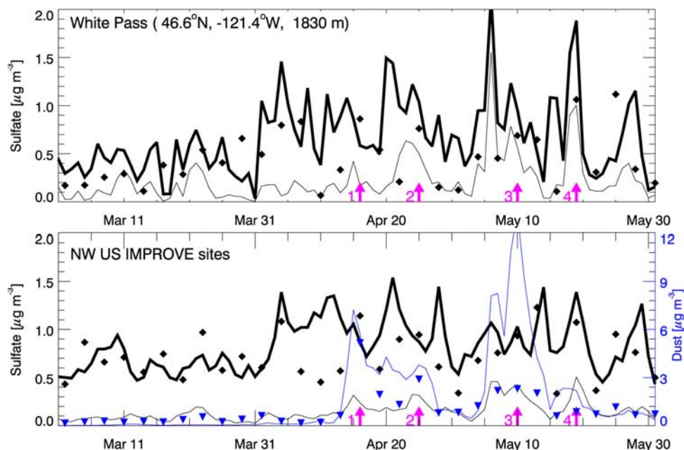
Figure 7. Time series of sulfate concentrations in surface air (top) at White Pass, Washington, and (bottom) for the ensemble of IMPROVE sites in the NW United States (west of 100^{\circ}\text{W} and north of 40^{\circ}\text{N} ). The IMPROVE observations are shown as diamonds, and the GEOS-Chem model values are shown as thick solid lines; correlation between the two is discussed in the text. The Asian anthropogenic contribution in GEOS-Chem is shown as thin black lines. Figure 7 (bottom) also shows dust concentrations observed at the IMPROVE sites (blue inverted triangles) and simulated by the GEOS-Chem model (thin blue line). Events of transpacific sulfate transport as seen at Midway (see Figure 2) and discussed in the text are highlighted with purple arrows.
