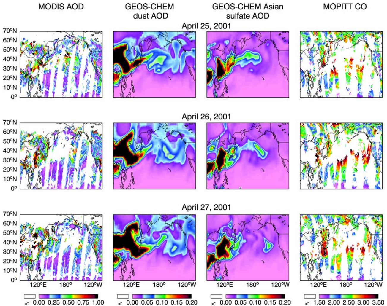
Figure 9. Transpacific sulfate event of April 2001 (event 2 in Figures 2 and 7). MODIS AODs (550 nm) are compared to the GEOS-Chem dust and sulfate AODs and to the CO columns observed by MOPITT ( \times 10^{18} molecules \text{cm}^{-2} ). Color scales are saturated at maximum values.
