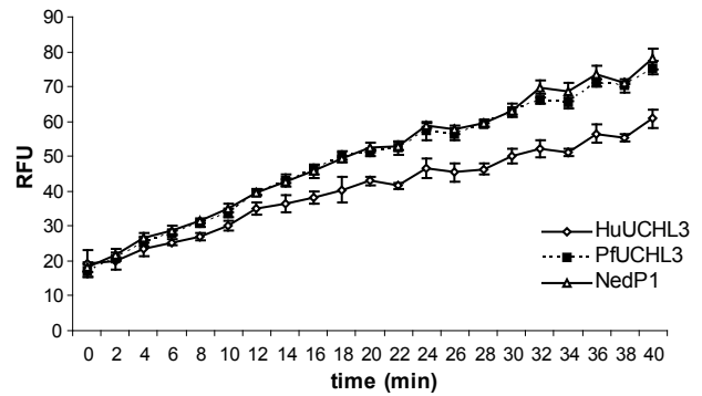
Nedd8-AMC (1.25uM) cleavage by 100pM enzyme
