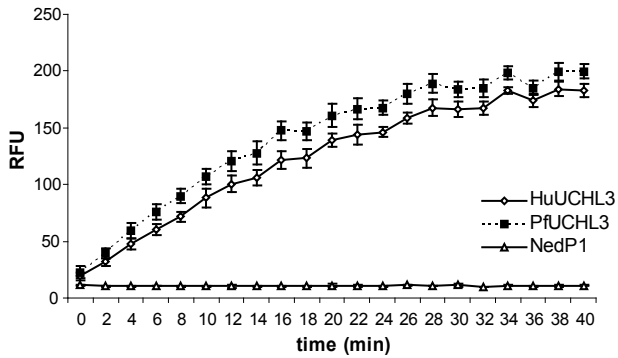
Ub-AMC (250nM) cleavage by 100pM enzyme
