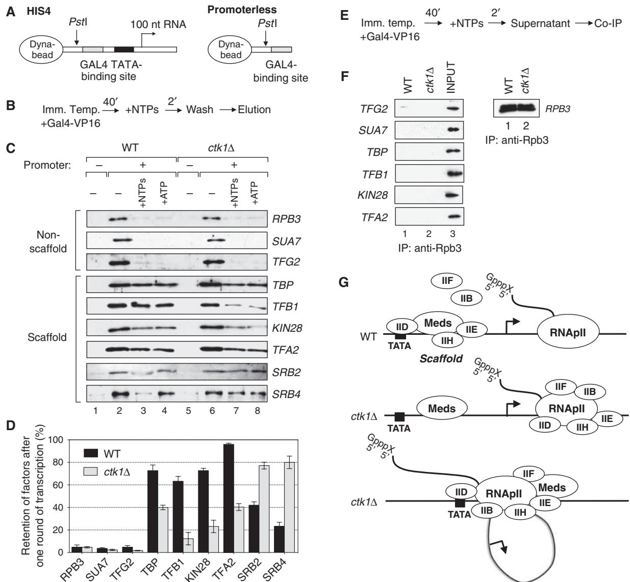
Figure 5 Ctk1 is required for the stability of the scaffold. (A) Immobilized templates used in this study. The HIS4 template contains a single Gal4 DNA-binding site upstream of the HIS4 core promoter containing a TATA box and transcription start site. The Promoterless template retains the Gal4 DNA-binding site but lacks the HIS4 promoter. Templates were immobilized on magnetic Dynabeads. (B) The scaffold formation assay. Cell extracts were incubated with the immobilized templates and activator Gal4-VP16 for 40 min. For single round measurement of transcription, PICs were incubated with NTPs for 2 min. (C) Immobilized templates were incubated with the activator Gal4-VP16 and yeast whole cell extracts from either WT (YSB726) or ctk1Δ (YSB854) for 40 min. After the formation of PICs, either nucleotides or ATP was added and incubated for 2 min. The templates were then washed and isolated by digestion with Pst I and detected by western blot. Lanes 1 and 5 show the controls for non-specific binding without promoter. Lanes 2 and 6 show typical PIC formation at the promoter. (D) Efficiency of scaffold formation was measured by quantitation of band intensities from lane 3 or 7 in WT and ctk1Δ cells (ImageJ v1.32). Signals from lane 2 or 6 were used as a control for each quantitation. Error bars are from three independent repetitions. (E) The scaffold assay after transcription termination. The cell extracts from either WT (YSB726) or ctk1Δ (YSB854) were incubated with the HIS4-immobilized templates and Gal4-VP16 for 40 min. To measure the association between RNApII and the basal transcription factors after termination, the supernatant was removed after incubation with NTPs for 2 min and immunoprecipitated with anti-Rpb3 antibody. (F) Coimmunoprecipitated proteins with Rpb3 from WT and ctk1Δ cells were determined by western blot using antibodies against non-scaffold (Tfg2 or Sua7) and scaffold components (TBP, Tfb1, Kin28, or Tfa2). (G) Model for the dissociation of basal transcription factors from elongating RNApII. See discussion for details.
