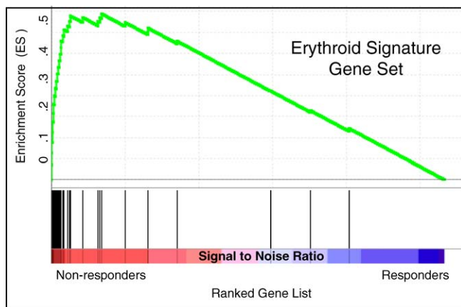
Figure 3. Gene Set Enrichment Analysis Using the Response Signature. Expression of the response signature, defined in the training set of samples, was analyzed in an independent test set of samples from MDS patients without 5q deletions. GSEA is a nonparametric statistical methodology that examines whether a set of genes, e.g., the response signature, occur towards the top of a list of genes that is ranked according to a class distinction. In this case, all genes on the microarray were ranked by signal-to-noise ratio in order of their differential expression between non-responders and responders. Black bars at the bottom of the figure indicate the location of genes in the response signature within the ranked list. The running enrichment score is shown in green. Nearly all of the genes in the erythroid response are expressed more highly in the non-responder class and are at the top of the ranked list of genes, resulting in a strong and statistically significant enrichment score ( p < 0.001 ). doi:10.1371/journal.pmed.0050035.g003
