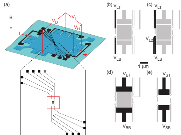
FIG. 1: (a) Device layout, showing leads used for current bias I and diagonal voltage, \nu_D , as well as bulk longitudinal and Hall voltages. (b-e) Gate layouts for 1 \mu\text{m} , 750 \text{ nm} , 2 \mu\text{m} , and 1.4 \mu\text{m} constrictions, indicating depleted (black) and grounded (gray) gates.
