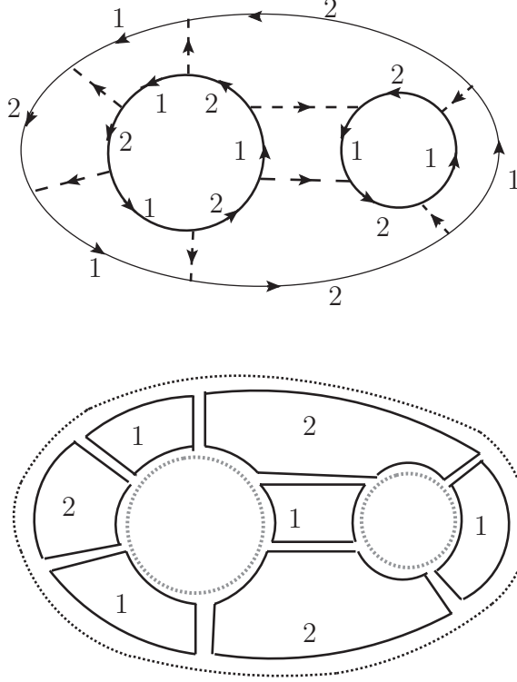
FIG. 16. Converting vacuum energy diagrams into surfaces: a face is attached to each solid and grey loop in the double-line representation (on the right). In the present case, the resulting surface is a sphere.
