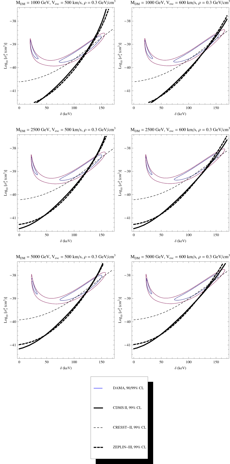
Figure 2: Allowed regions for fits of inelastic dark matter to the DAMA data, as well as constraints from CDMS II, CRESST-II, and ZEPLIN-III. We fix the local DM density at \rho = 0.3 \text{ GeV}/\text{cm}^3 , and vary the DM mass and escape velocity. These plots assume the relation f_p = f_n .
