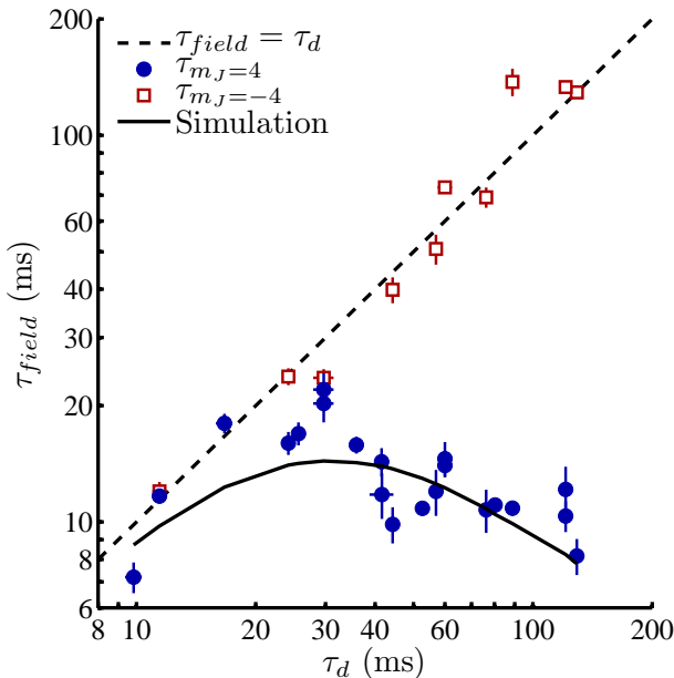
FIG. 6: (color online) Nickel m_J = J and m_J = -J lifetimes in a 0.8 Tesla field vs. diffusion lifetime. The dashed line was drawn with a slope = 1 to demonstrate that the m_J = -J atoms leave the cell by diffusion as expected. The m_J = J atoms decay quickly due Zeeman relaxation in the region of high \tau_d . The best fit of the m_J = J data to a finite temperature Zeeman cascade simulation yields a value of \gamma = 5 \times 10^3 .
