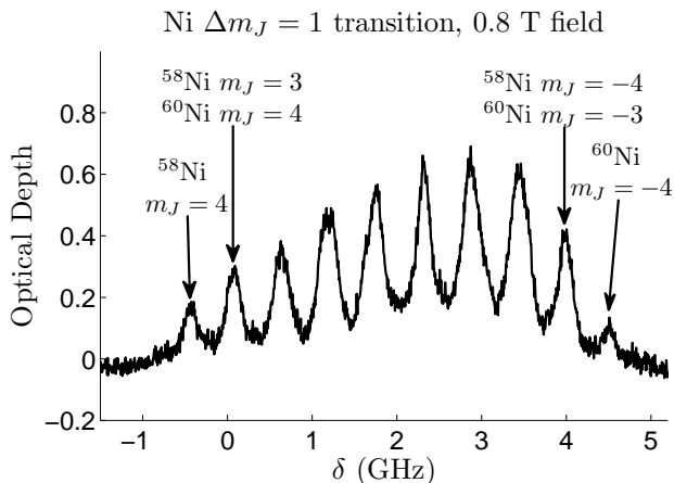
FIG. 2: Nickel optical depth vs. frequency (arbitrary zero) in a homogeneous (Helmholtz) field. Each isotope has 9 lines corresponding to the 9 m_J states. The Zeeman and isotope shifts are roughly equal at 0.8 T fields, causing lines of different isotopes to overlap. Measurements of the m_J = J state lifetime are performed by parking on the m_J = 4 transition peak and measuring the optical depth vs. time.
