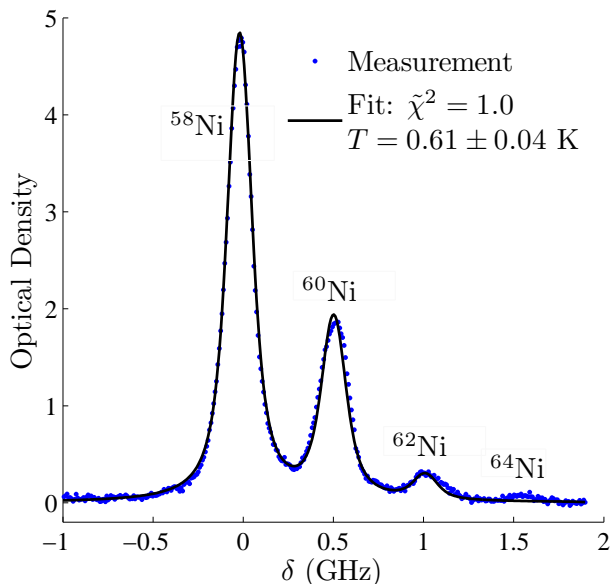
FIG. 4: (color online) Nickel zero-field optical depth vs. frequency 50 ms after ablation. Frequency zero set to ^{58}\text{Ni} resonance. Temperature and density are found by fitting to a Voigt profile.
