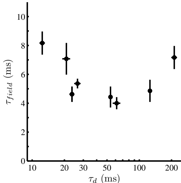
FIG. 7: Iron m_J = J lifetimes in a 1.0 Tesla field vs. diffusion lifetime at zero field. There is no region of \tau_d for which \tau_J increases. This indicates that Zeeman relaxation is the dominant loss mechanism for the entire range of data.
