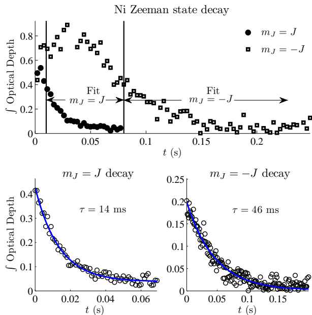
FIG. 3: (color online) Nickel m_J = J and m_J = -J optical depth (integrated over the atomic line) vs. time. Upper plot shows Zeeman state evolution starting immediately after laser ablation. The m_J = -J state experiences an initial increase in optical depth because m_J \neq -J states are relaxing into the m_J = -J state. Lifetime fits are performed over the indicated regions. Lower left(right) plot shows m_J = J(-J) lifetime fit.
