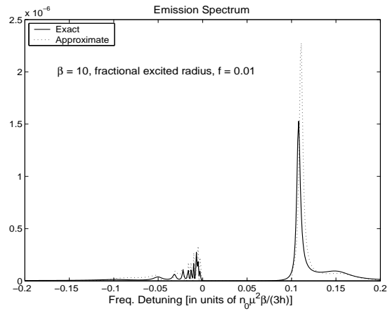
FIG. 5. Same as Fig. 4(a), except (a) \beta = 10 , f = 1 and (b) \beta = 10 , f = 0.01 .
