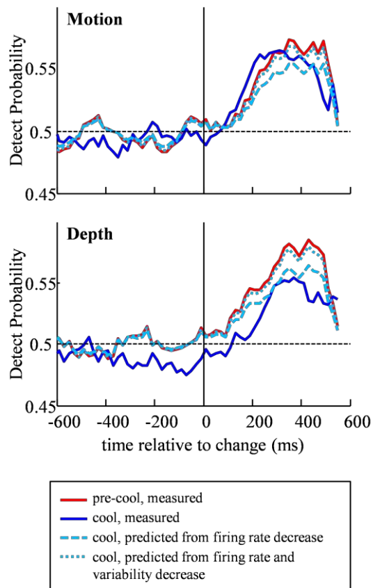
Figure 27: DP prediction
