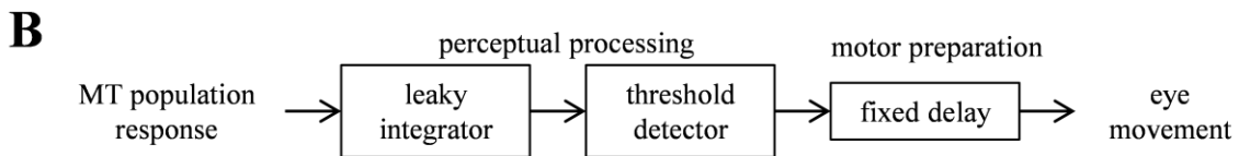
Figure 29: Threshold model
