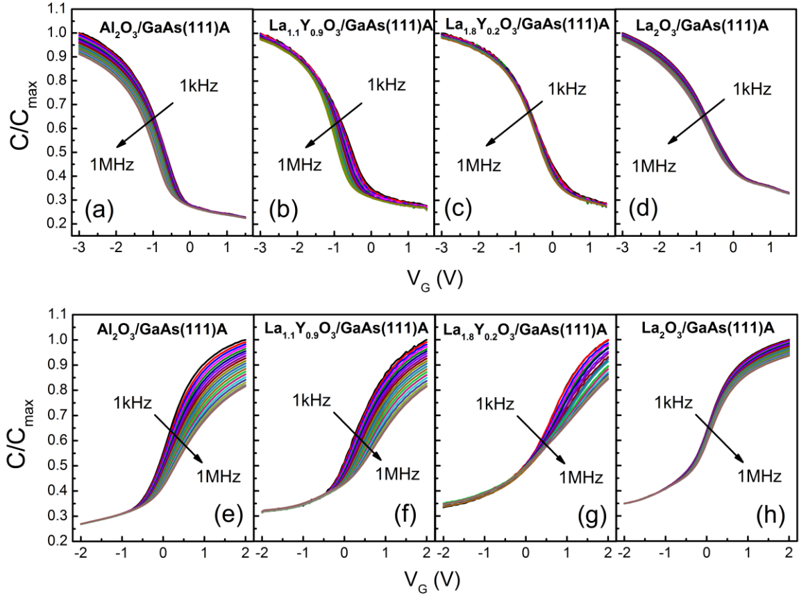
Figure 3. C - V characteristics of p-type and n-type GaAs MOS capacitors with stacks of (a, e) Ni/8nm \text{Al}_2\text{O}_3/\text{GaAs}(111)\text{A} , (b, f) Ni/6.5 nm \text{Al}_2\text{O}_3/7.5 nm \text{La}_{1.1}\text{Y}_{0.9}\text{O}_3/\text{GaAs}(111)\text{A} , (c, g) Ni/6.5 nm \text{Al}_2\text{O}_3/7.5 nm \text{La}_{1.8}\text{Y}_{0.2}\text{O}_3/\text{GaAs}(111)\text{A} , and (d, h) Ni/6.5 nm \text{Al}_2\text{O}_3/9 nm \text{La}_2\text{O}_3/\text{GaAs}(111)\text{A} , respectively.
