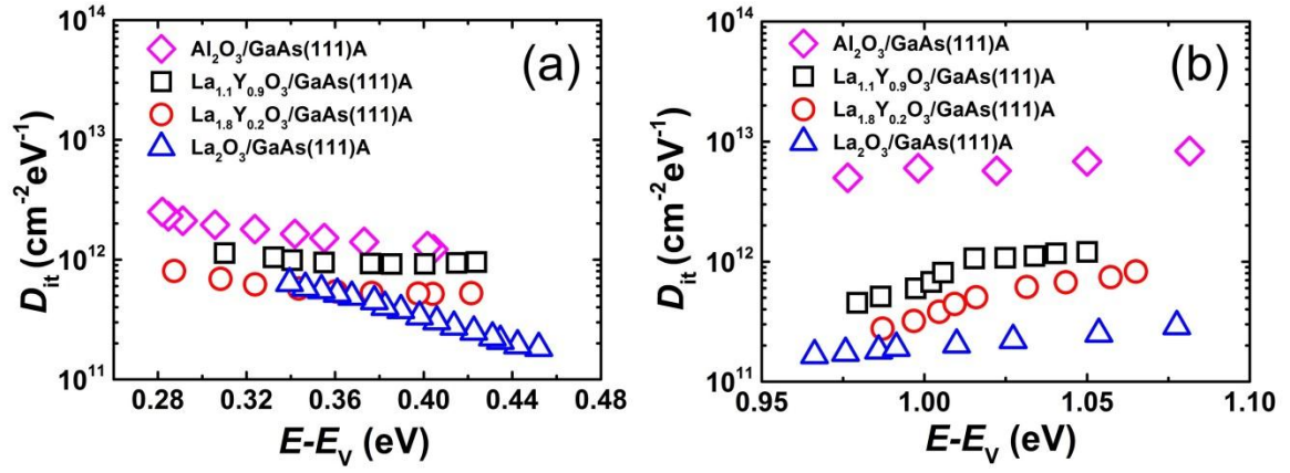
Figure 4. D_{it} distribution in the GaAs band gap obtained on both (a) p-type and (b) n-type MOS capacitors with Al 2 O 3 /GaAs(111)A, La 1.1 Y 0.9 O 3 /GaAs(111)A, La 1.8 Y 0.2 O 3 /GaAs(111)A and La 2 O 3 /GaAs(111)A as the interfaces, respectively.
