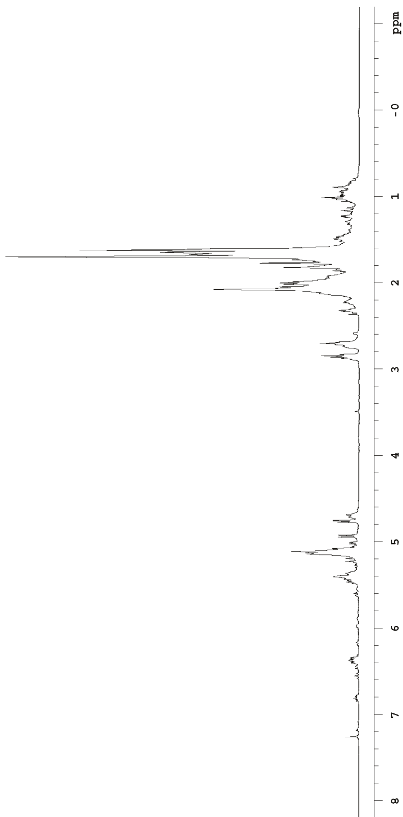
NMR 22: 1 H NMR spectrum (500 MHz, CDCl 3 , 25 °C) of farnesene ( α-isomer ) (ex. 10)
