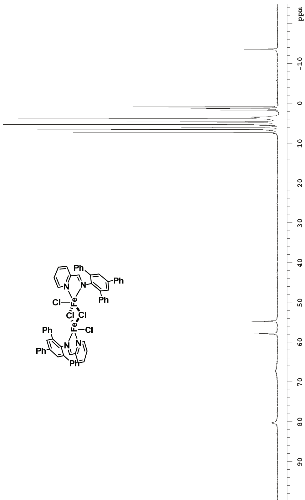
NMR 7: ^1\text{H} NMR spectrum (500 MHz, \text{CDCl}_3 , 25\text{ }^\circ\text{C} ) of 2
