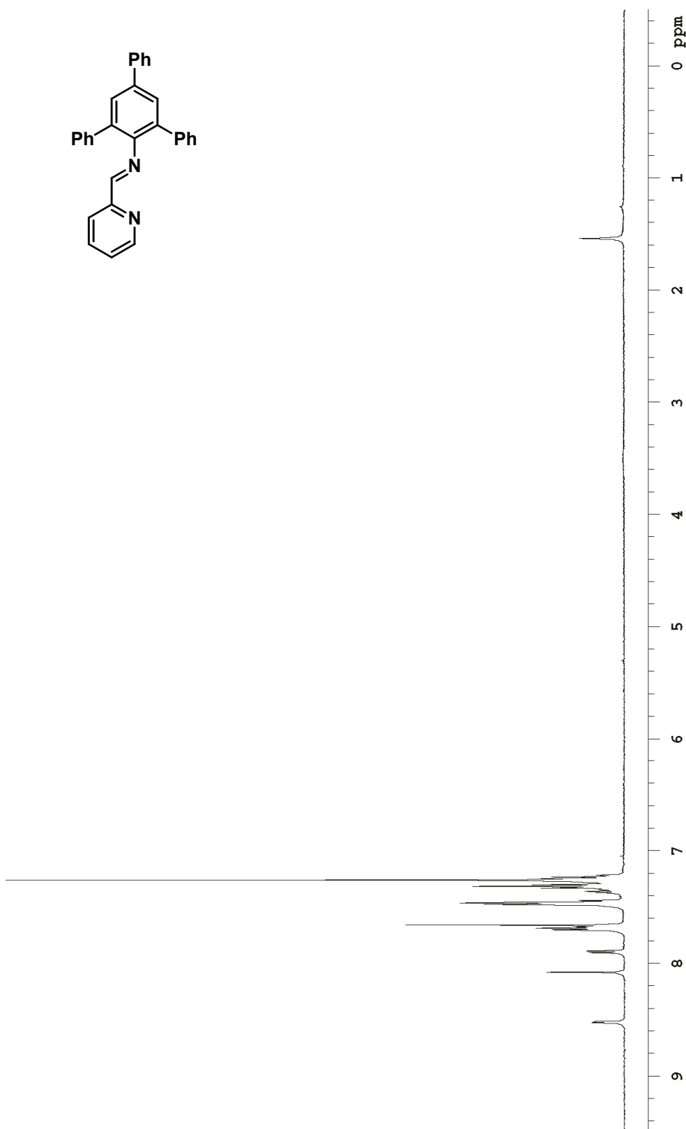
NMR 5: ^1\text{H} NMR spectrum (500 MHz, \text{CDCl}_3 , 25 ^\circ\text{C} ) of S2
