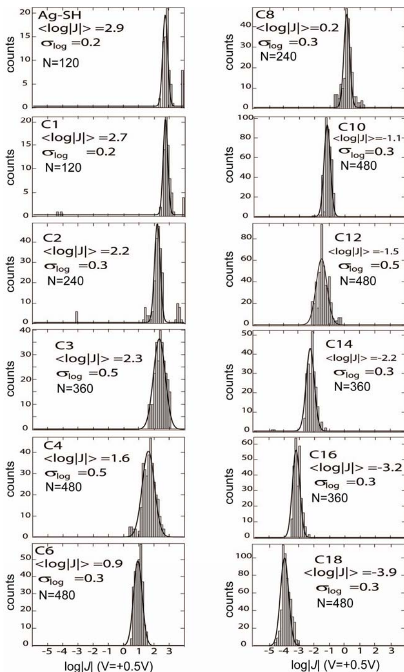
Figure 4. Histograms showing the distributions of values of \log|J| at V=+0.5V across Ag^{TS} -SAM// Ga_2O_3 /EGaIn junctions using flattened conical tips. With “Cn” we indicate SAMs of alkanethiolates with n carbon atoms. Solid curves represent Gaussian fits. N is the number of data points. Data collected using the 1/3/20 protocol. No data were excluded. The heights of the bars of the histograms count the number of points (counts) with values of \log|J| within the width (0.13) of the bars. For each distribution, the value of Gaussian mean, median, and mode (the value of \log|J| with the highest bar) differed by less than 0.1.
