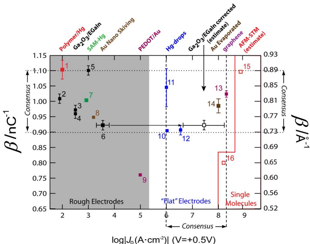
Figure 8. Plot of values of \beta versus values of \log|J_0(V=+0.5V)| reported (filled dots) or estimated (empty squares) for tunneling through n -alkanethiolates with junctions using top-electrodes indicated on the top-axis. Numbering from Table 1. The horizontal arrowed line points to the value of J_0 for \text{Ag}^{\text{TS}}\text{-SAM//Ga}_2\text{O}_3/\text{EGaIn} corrected for the value of the effective electrical contact area ( A_{\text{elec}}=10^{-4\pm 0.5}\cdot A_{\text{geo}} ); the horizontal error bar of this estimate incorporates the uncertainties on the estimation of J_0 from tunneling across SAMs, and on the estimation of the effective electrical contact area. Junctions grouped in the gray zone use either rough top-electrodes, or rough bottom-electrodes.
