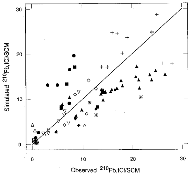
Fig. 4a. Scatterplot of simulated versus observed yearly mean 210 Pb concentrations at 85 sites around the world for which at least one full year of observations is available. The 1:1 line is also shown. Site locations and references are given in Figure 5a.
