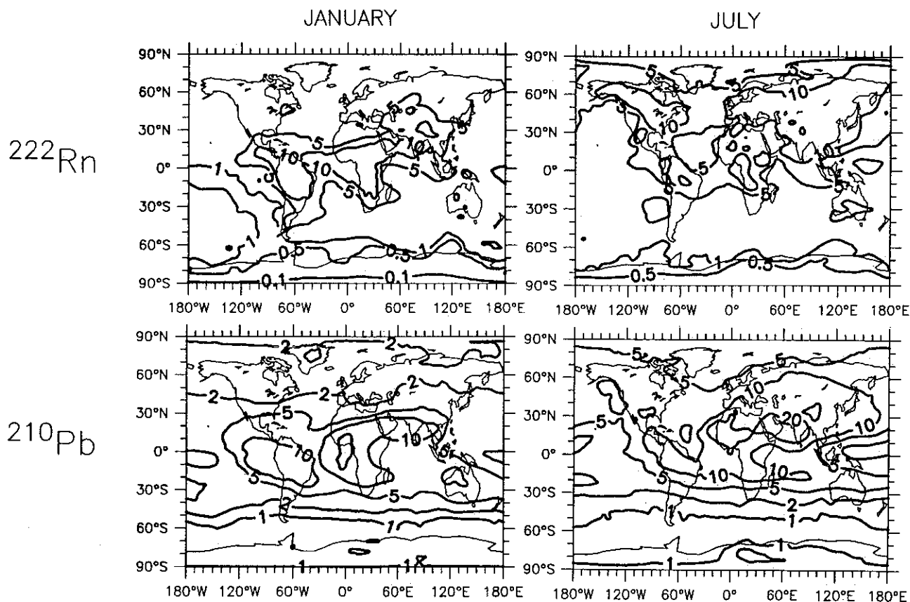
Fig. 3b. Monthly mean concentrations of ^{222}\text{Rn} ( \text{pCi}/\text{m}^3 STP) and ^{210}\text{Pb} ( \text{fCi}/\text{m}^3 STP) at 6-km altitude in the model for January and July.
