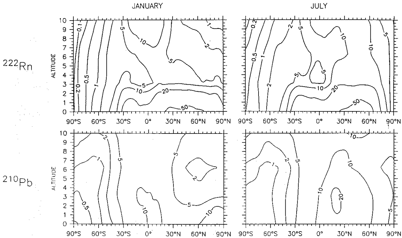
Fig. 3c. Zonal mean concentrations of 222 Rn (pCi/m 3 STP) and 210 Pb (fCi/m 3 STP) as a function of altitude and latitude in the model for January and July.
