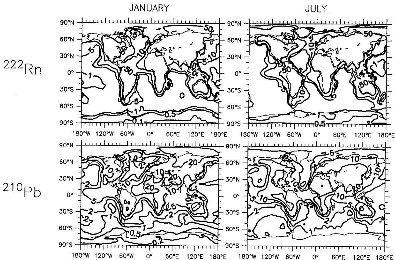
Fig. 3a. Monthly mean concentrations of ^{222}\text{Rn} ( \text{pCi}/\text{m}^3 STP) and ^{210}\text{Pb} ( \text{fCi}/\text{m}^3 STP) in surface air in the model for January and July.
