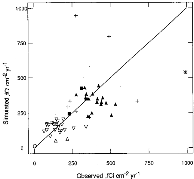
Fig. 4b. Scatterplot of simulated versus observed yearly mean total deposition fluxes of 210 Pb at 55 sites around the world for which at least one full year of observations is available. The 1:1 line is also shown. The measurements are from open buckets and soil inventories. Site locations and references are given in Figure 5b.
