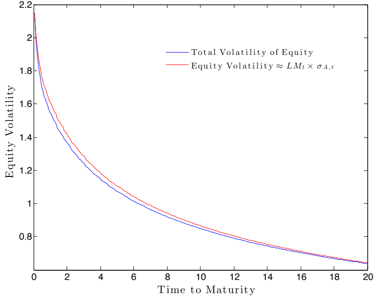
Figure 18: Equity Volatility Analysis in SVJ Model
