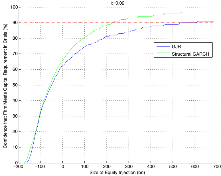
Figure 12: Precautionary Capital: Bank of America on 10/1/2008
