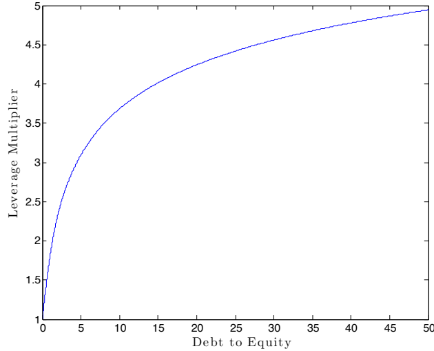
Figure 1: BSM Leverage Multiplier
