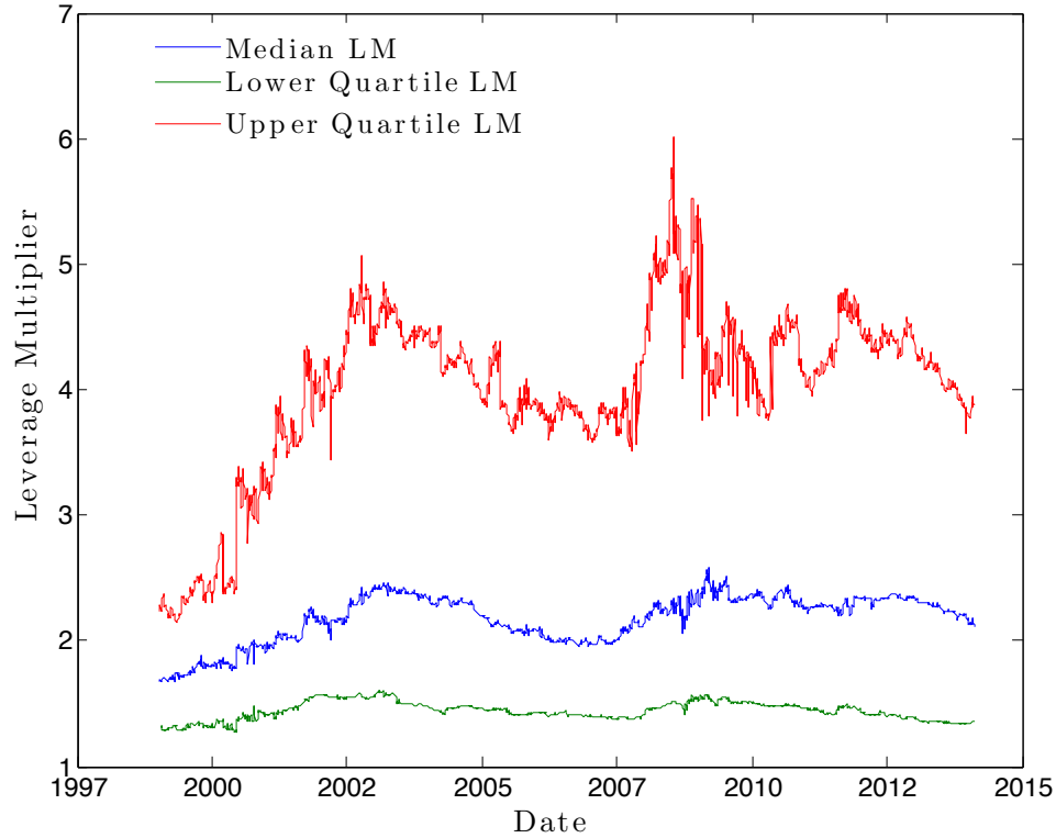
Figure 7: Time Series of Leverage Multiplier Across Quartiles
