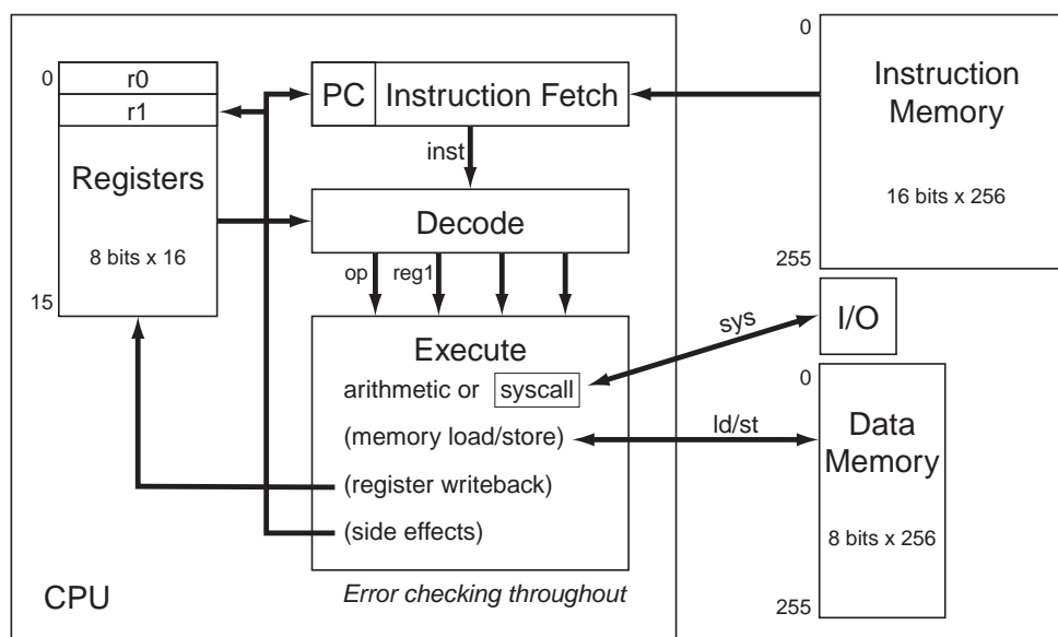
Figure 2: A block diagram of the ANT architecture.
