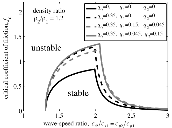
Figure 5. Regions of instability for a density ratio of 1.2. The solid black line corresponds to the case of no poroelastic response and the dashed black line is for the case with the response included, assuming that poroelastic properties are homogeneous. Adding the poroelastic effect stabilizes sliding over a larger range of friction coefficients. Cases for which one side is more permeable than the other are shown by the solid gray and dashed gray lines. When the stiff side is more permeable, the poroelastic effect opposes the elastic bimaterial effect and the region of stability expands (solid gray line). When the compliant side is more permeable, the poroelastic and elastic bimaterial effects act in concert and the region of stability diminishes (dashed gray line).
