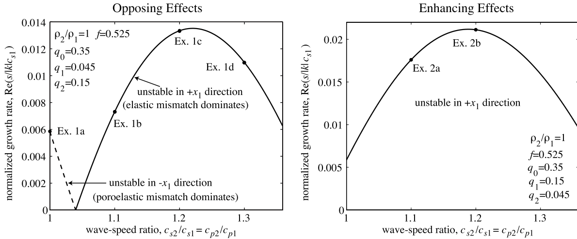
Figure 4. Growth rate of the unstable mode for (left) opposing poroelastic and elastic effects with the stiff side more permeable and (right) enhancing poroelastic and elastic effects with the compliant side more permeable.
