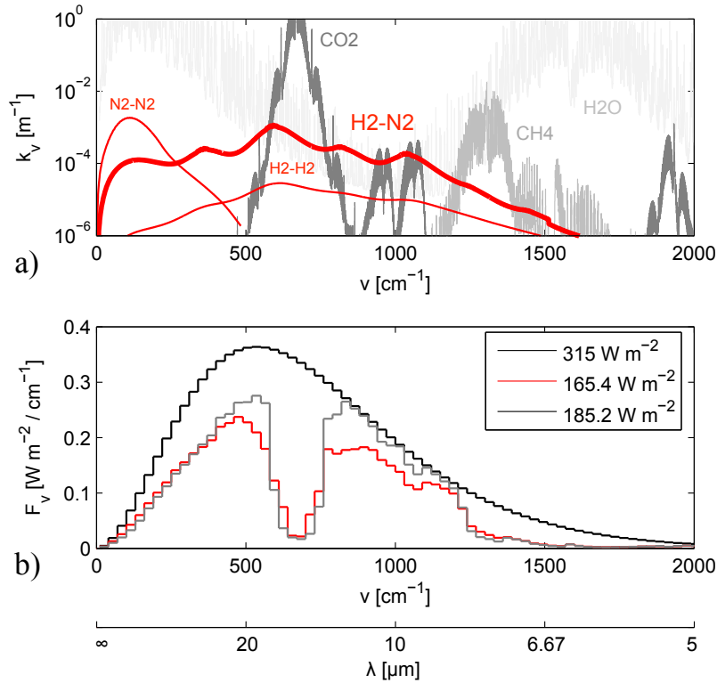
Figure 1: a) Infrared absorption at the surface for an Archean atmosphere with \times 3 PAL \text{N}_2 , 10% \text{H}_2 , 1700 ppm \text{CO}_2 ( \sim 10\times PAL), 5 ppm \text{CH}_4 , surface temperature 273 K and relative humidity 0.77. b) Corresponding outgoing longwave radiation (OLR) assuming line absorption only (gray line) and with CIA included (red line). Black line shows the blackbody emission at 273 K, while the numbers in the box show the integrated OLR for each case. See SOM for calculation details. Given high atmospheric hydrogen and nitrogen levels, \text{H}_2\text{-N}_2 absorption dominates in the 750\text{--}1200\text{ cm}^{-1} spectral region where the bands of the other greenhouse gases are relatively weak.
