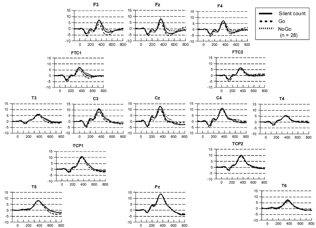
Fig. 1. Grand averaged waveforms for each task. Note the bilateral fronto-central reduction and left-less-than-right asymmetry of P300 in the Go task, and the equivalence of all 3 tasks at Pz.
