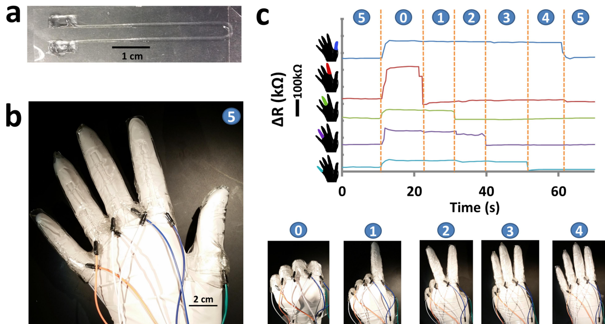
Figure 5. An example of a printed hydrogel-elastomeric type device, where fairly arbitrary shapes and designs can be easily integrated into the system by virtue of the printing process. In this case a) a simple resistance-based strain gauge is replicated using the hydrogel as the conductor and PDMS as the encapsulating substrate. b) By attaching the sensor to a flexible glove and flexing the digit we are able to observe a change in resistance up to 30% of its initial value at maximum finger bending and c) illustrate this process for a variety of hand gestures for each digit's strain sensor resistance change over time.
