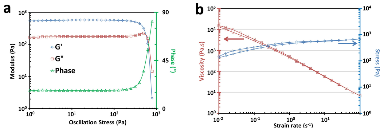
Figure 2. Rheological analyses of the rheological modifier for the hydrogel precursor. a) Typical oscillatory rheology results showing shear storage ( G' ) and shear loss ( G'' ) moduli evolution of inks used over increasing shear stress. b) Typical viscometry results showing stress and viscosity against shear rate. Tests were begun at low shear rates and swept up, then back down to demonstrate a mild thixotropic effect.
