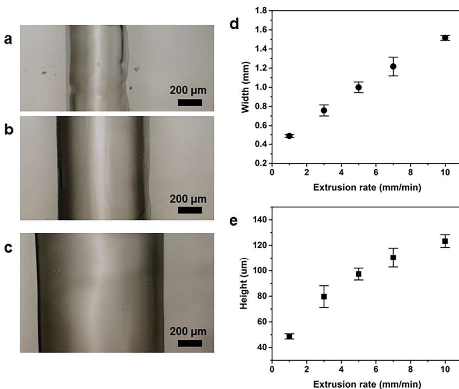
Figure S1. Variations in hydrogel geometry by only nominal extrusion rate variation, keeping stage velocity (450 mm/min), extrusion height (300 μm) and extrusion tip diameter (337 μm) constant. We illustrate gel geometry with optical micrographs of the printed hydrogel on top of PDMS substrate at (a) 1, (b) 3, and (c) 5 mm min -1 extrusion rates. (d) shows a plot of the relationship between extrusion rate and final line width, with what appears to be a linear correlation. (e) A similar plot for final gel height versus extrusion rate.
