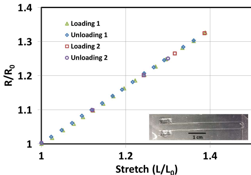
Figure S2. Resistance change of a stretched strain gauge sample, demonstrating a linearity of the resistance change response for this design up to 40% strain.
