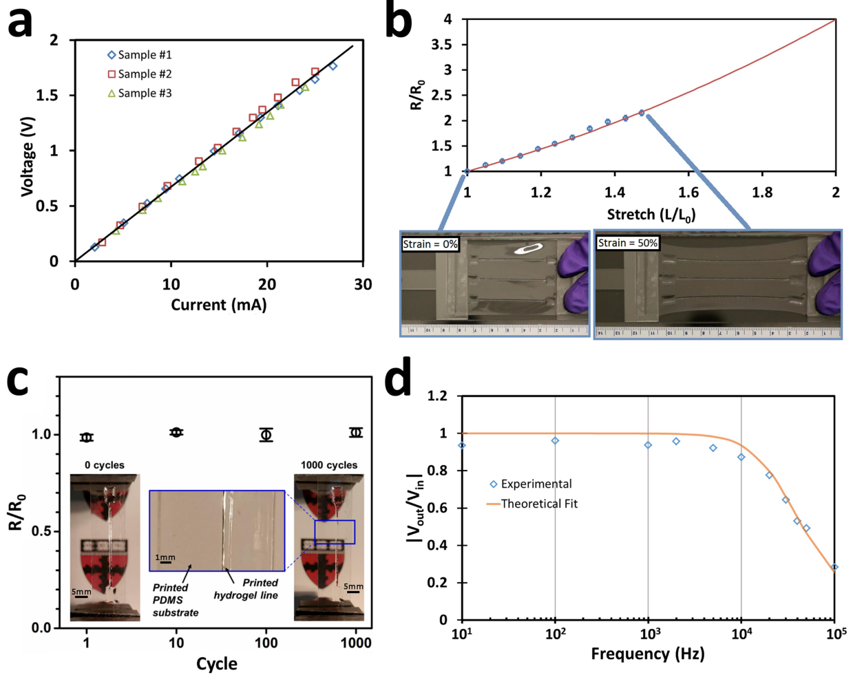
Figure 4. Electrical characterizations of the hydrogel in either bulk or printed state. a) I-V curves obtained from 4-point probe measurements performed on bulk hydrogel samples. Sample dimensions were on average 30 cm long, 4.2 mm wide, and 3.5 mm in height, with an average measured resistance of 67.3 \pm 2.4 \Omega ; this corresponds to a conductivity of 10.39 \pm 0.31 \text{ S m}^{-1} . b) The normalized resistance of printed hydrogels on a PDMS substrate is measured as a function of stretch, plotted against the ideal geometric behavior. Photos illustrate the sample in the initial (strain = 0%) state and the fully stretched (strain = 50%) state with the mechanical load applied only to the PDMS. c) The normalized resistance of printed hydrogels on a PDMS substrate as a function of fatigue cycle number. Uniaxial tensile strain cycles of 20% strain were performed for up to 1000 cycles. No significant change to the resistance vs. strain behavior was observed during our tests. Comparing images both before and after fatigue tests illustrate the lack of visible damage or delamination d) The transfer function of an ionic cable design is plotted against frequency. We perform a theoretical fitting of our results using a simple RC circuit model for the ionic cable and can observe a reasonable level of agreement between experimental results and theory.
