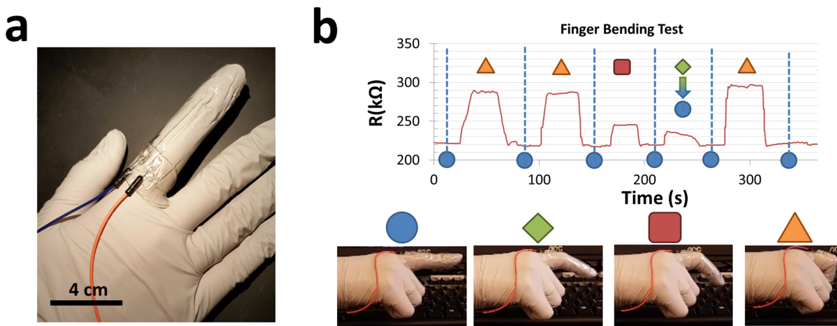
Figure S3. A single strain gauge is mounted onto the index finger and held in various positions while the resistance is recorded. (a) Illustrates the mounting of the strain gauge using VHB tape and leads connecting the gauge. (b) Illustrates the various positions alongside the time-trace of the gauge's resistance. The mildly bent position (green diamond) is gradually straightened to the default position, whereas others were more rapidly transitioned from straight to bent positions.
