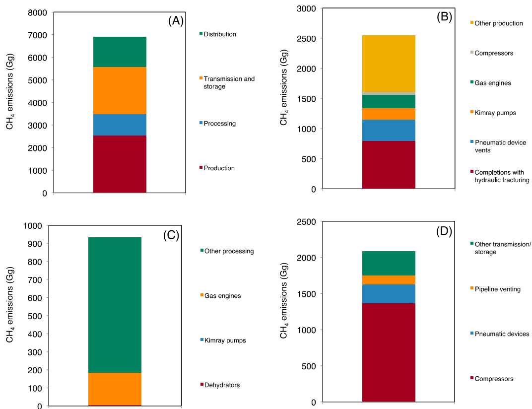
Fig. S1. CH 4 emissions from EPA 2011 inventory for the NG sector. (A) Total breakdown between four process stages. Sector specific breakdown for Production (B) , Processing (C) and Transmission and Storage (D) . Source: [table A-138 (32)].
