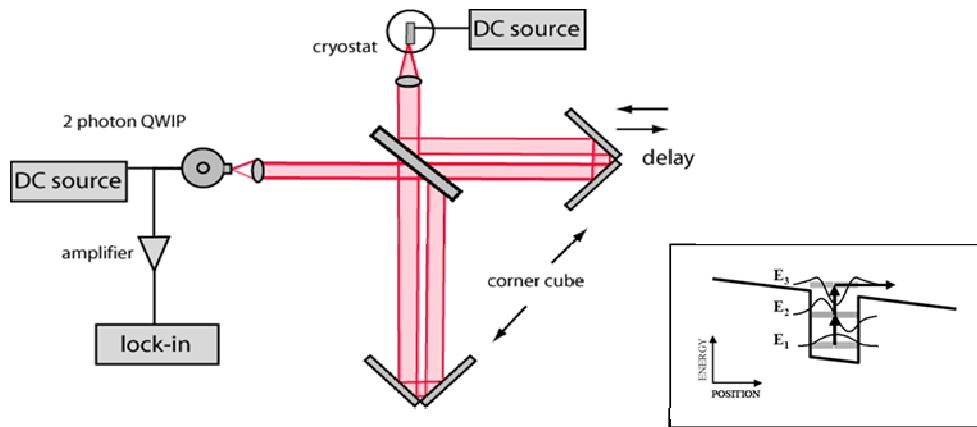
Fig. 5. The experimental setup for the autocorrelation measurement using two-photon QWIP. Inset: conduction band diagram of the two-photon QWIP showing three equidistant energy levels.
