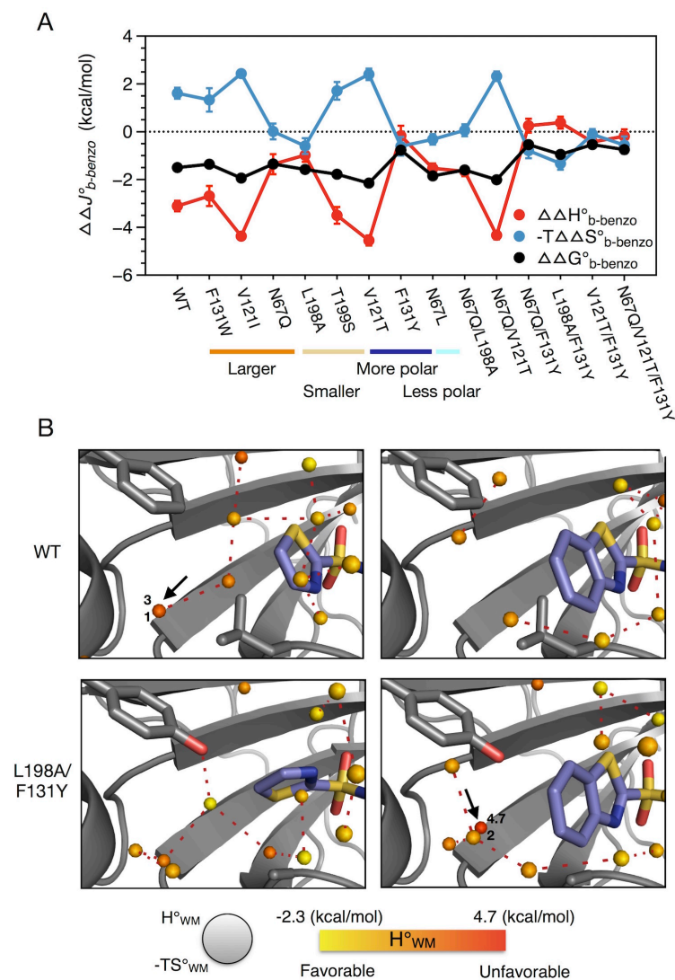
Figure 3. Hydrophobic association. (A) Differences in the thermodynamic binding parameters for BTA and TA ( \Delta\Delta J^{\circ}_{b-benzo} = \Delta J^{\circ}_{b-BTA} - \Delta J^{\circ}_{b-TA} ) reveal the thermodynamic signature of hydrophobic association between the benzo ring of BTA and the nonpolar wall of HCAII. (B) Results of WaterMap calculations for L198A/F131Y (colored as in Fig. 2C). In the wild-type, the binding of TA traps an enthalpically unfavorable water near the nonpolar wall (arrow); when BTA binds, its benzo ring releases this molecule and brings about an enthalpically favorable and entropically unfavorable rearrangement of water. In L198A/F131Y, mutations stabilize a network of water over the nonpolar wall. The binding of TA leaves much of this network intact,
