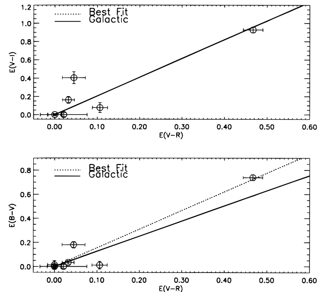
FIG. 5.—Measured ratio of color excesses from SN Ia's and the expectation for galactic dust. The two plotted ratios ( dotted line ) of color excesses are generally consistent with the ratios expected from galactic dust ( solid line ), but the results are strongly dependent on the highly reddened SN 1995E.
